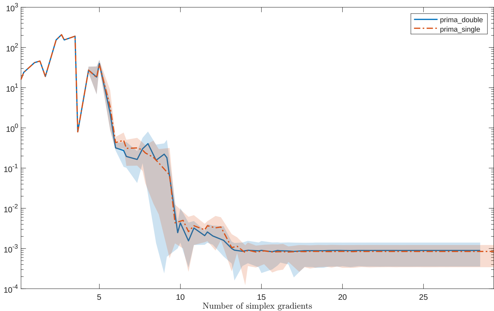
Solving "BROYDN3DLS" with "noisy_0.001_mixed_gaussian" feature
