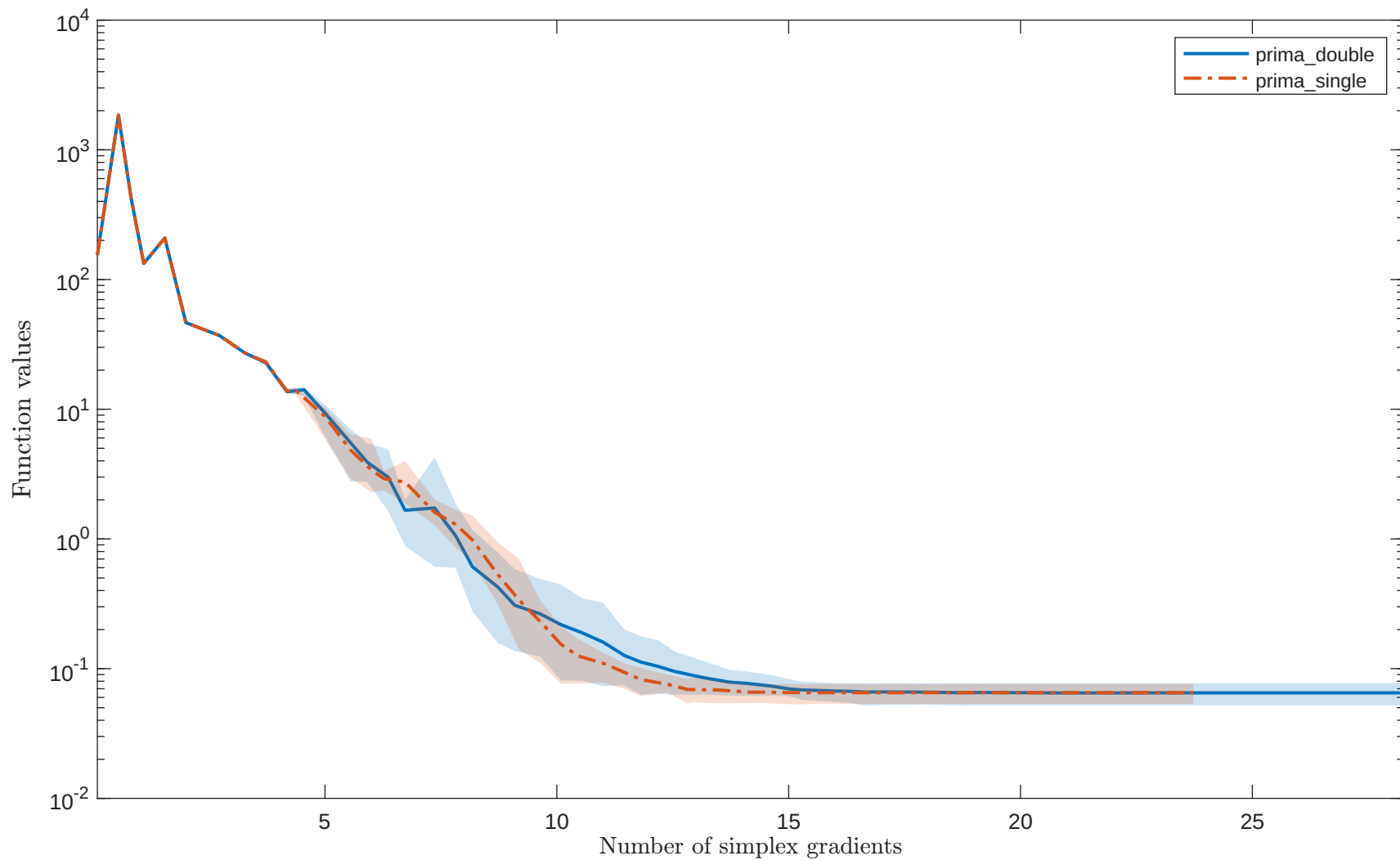
Solving “BROYDNBDLS” with “noisy_0.001_mixed_gaussian” feature
