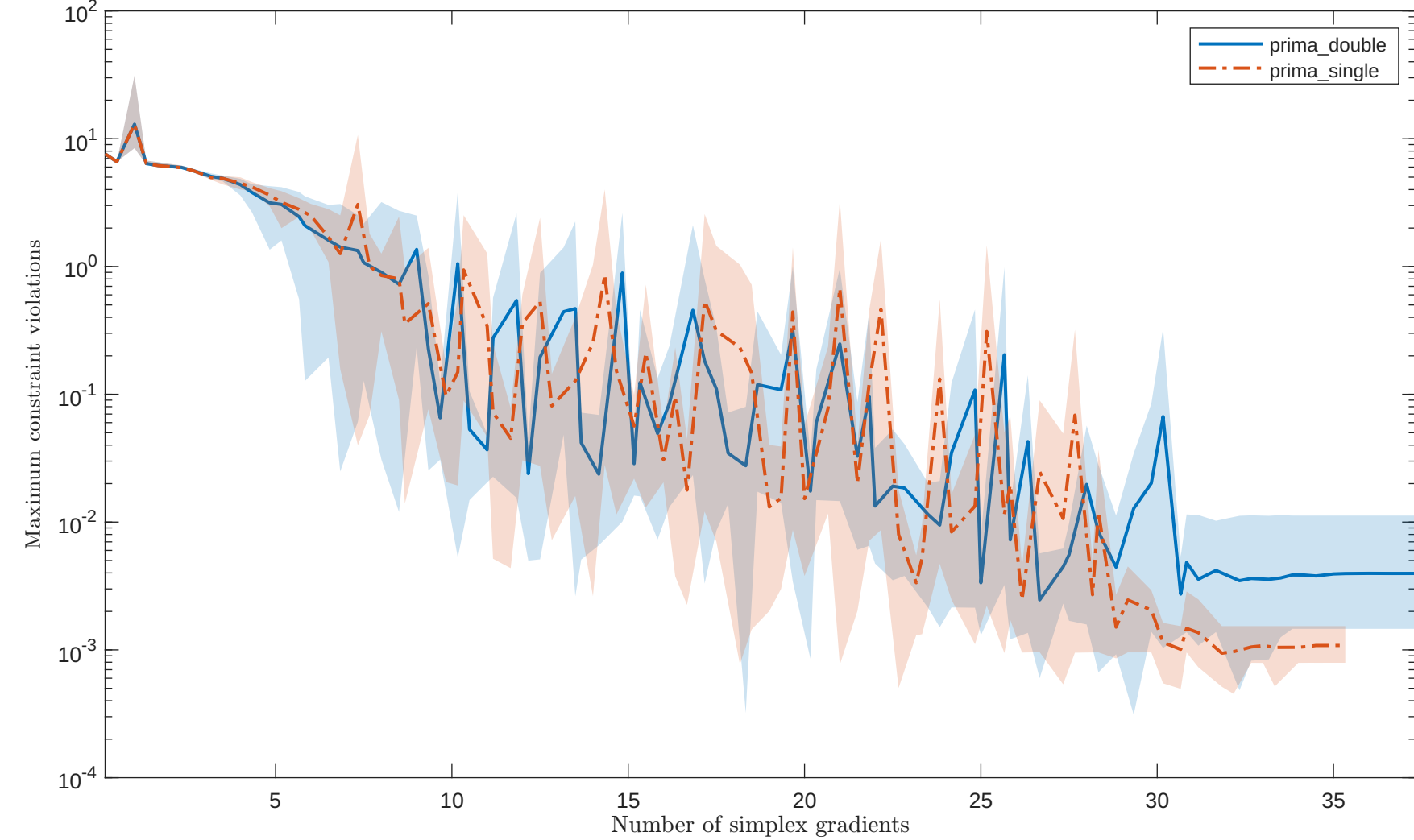
Solving "BT12" with "noisy_0.001_mixed_gaussian" feature
