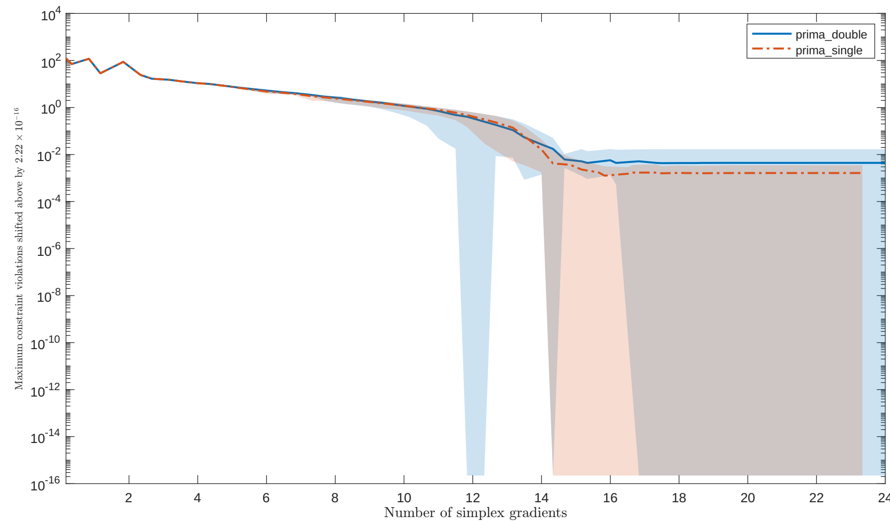
Solving "CANTILVR" with "noisy_0.001_mixed_gaussian" feature
