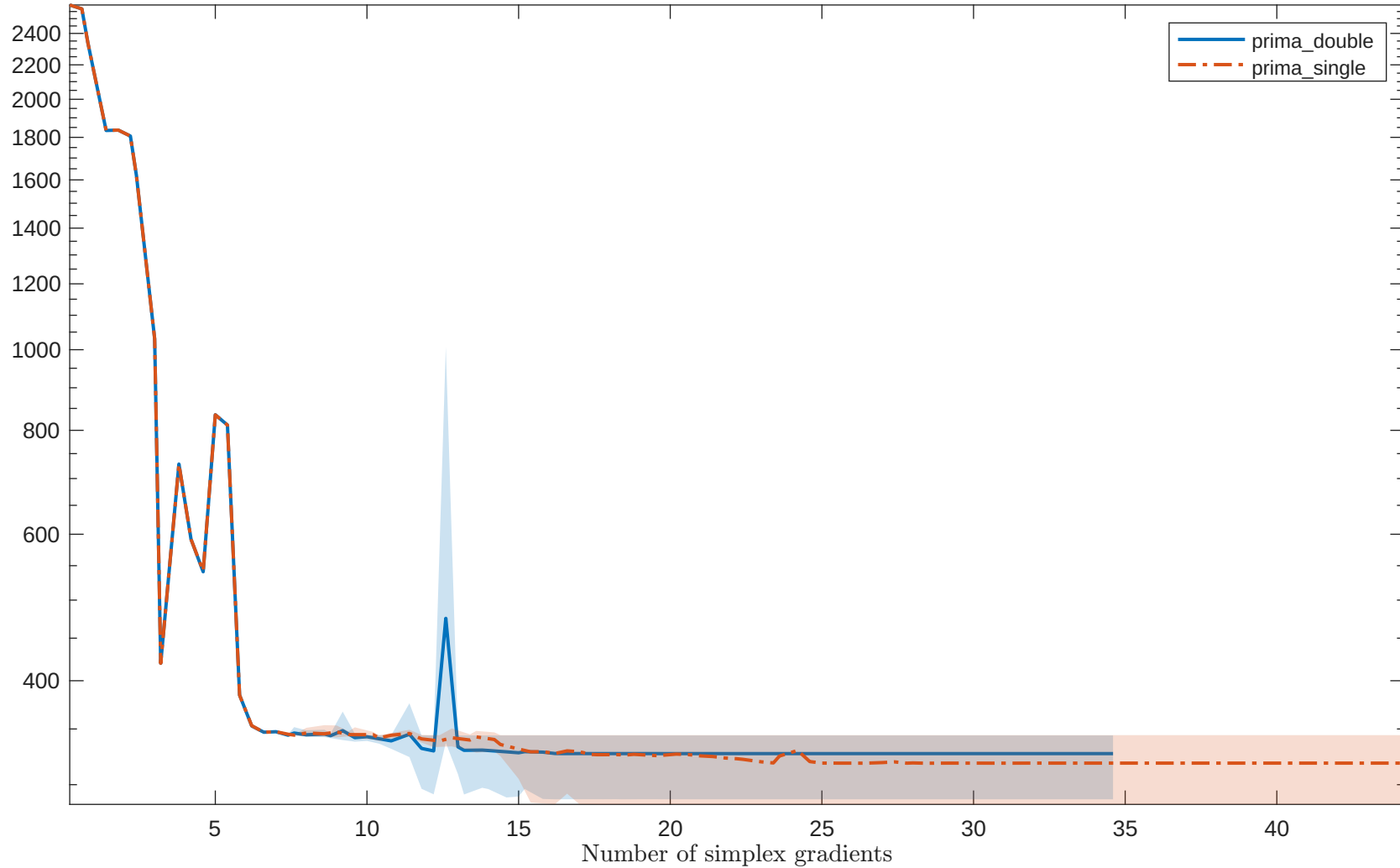
Solving "FREUROTH" with "noisy_0.001_mixed_gaussian" feature
