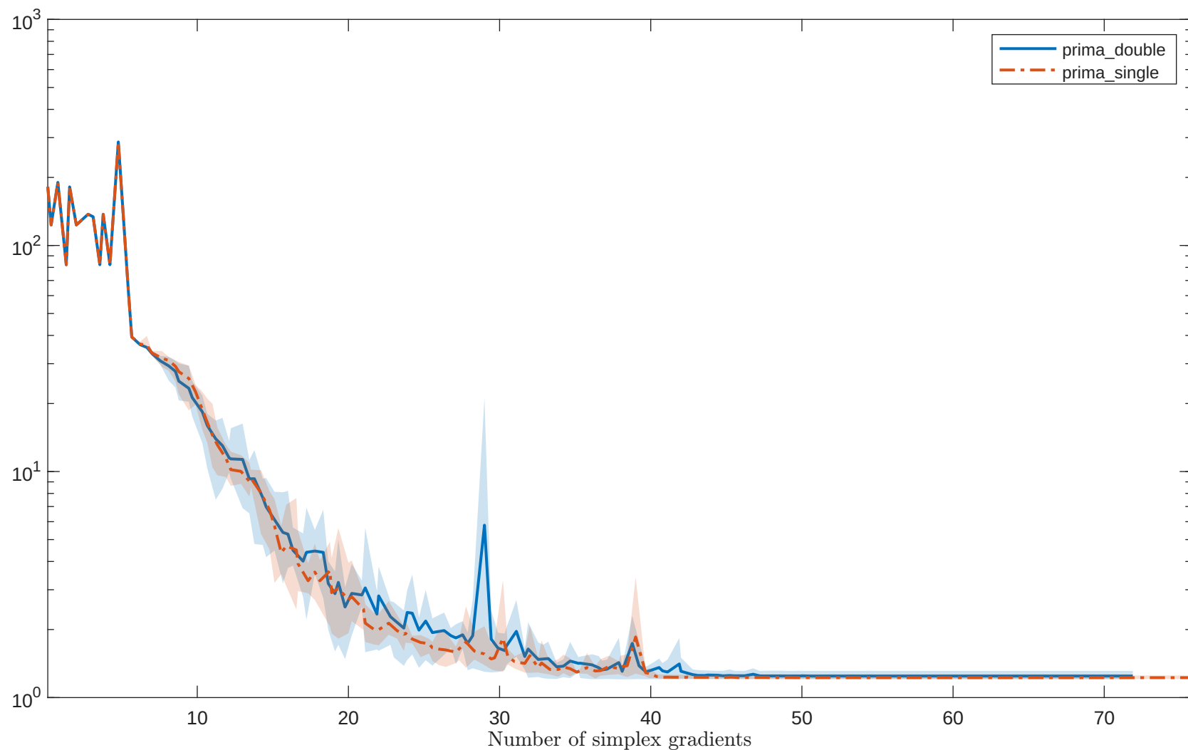
Solving “HEART8LS” with “noisy_0.001_mixed_gaussian” feature
