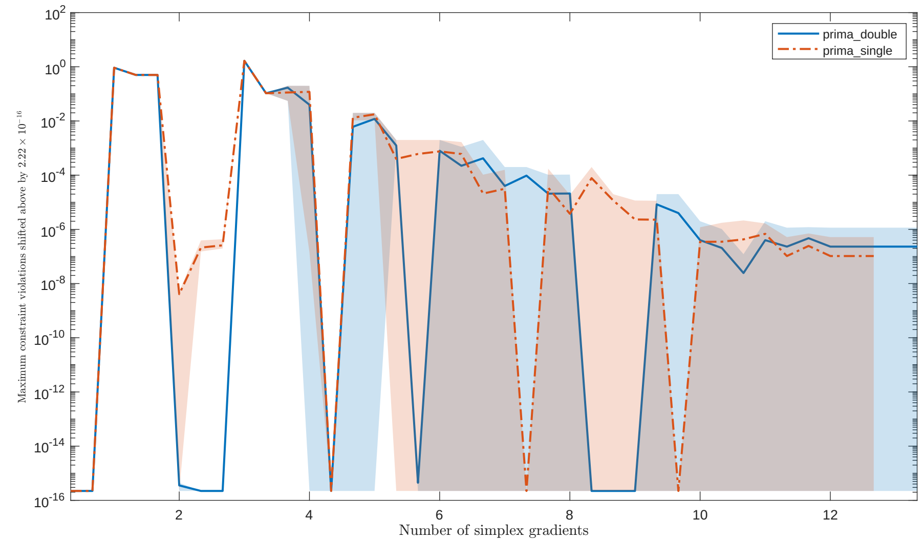
Solving “HS24” with “noisy_0.001_mixed.gaussian” feature
