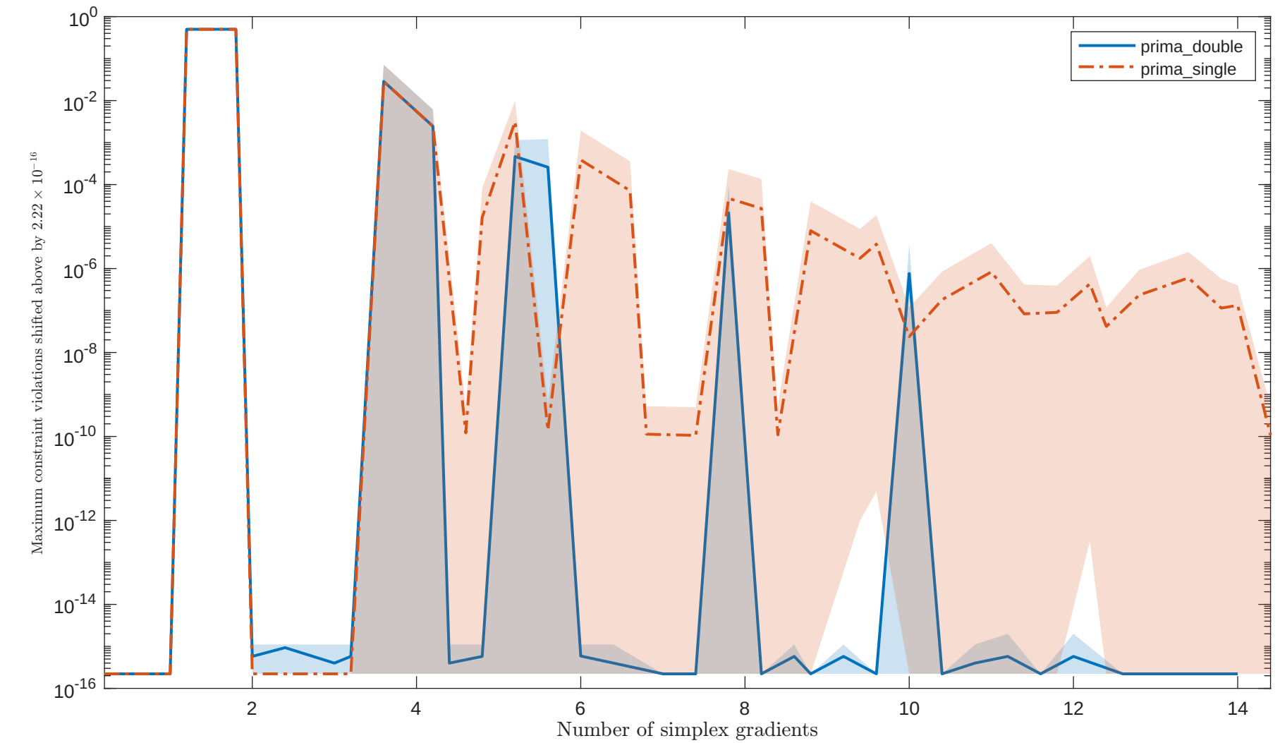
Solving "HS76I" with "noisy_0.001_mixed-gaussian" feature
