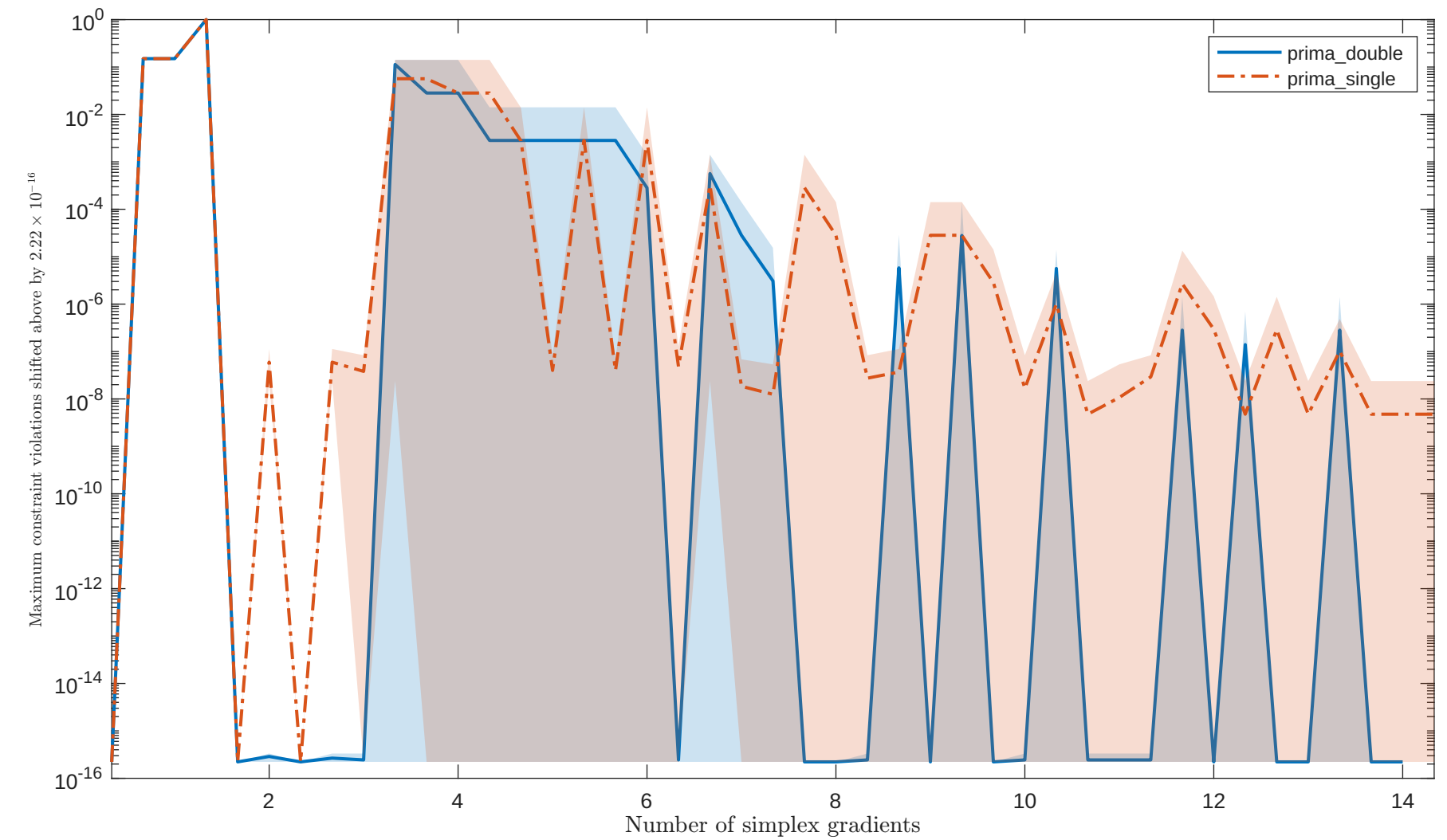
Solving “HUBFIT” with “noisy_0.001_mixed.gaussian” feature
