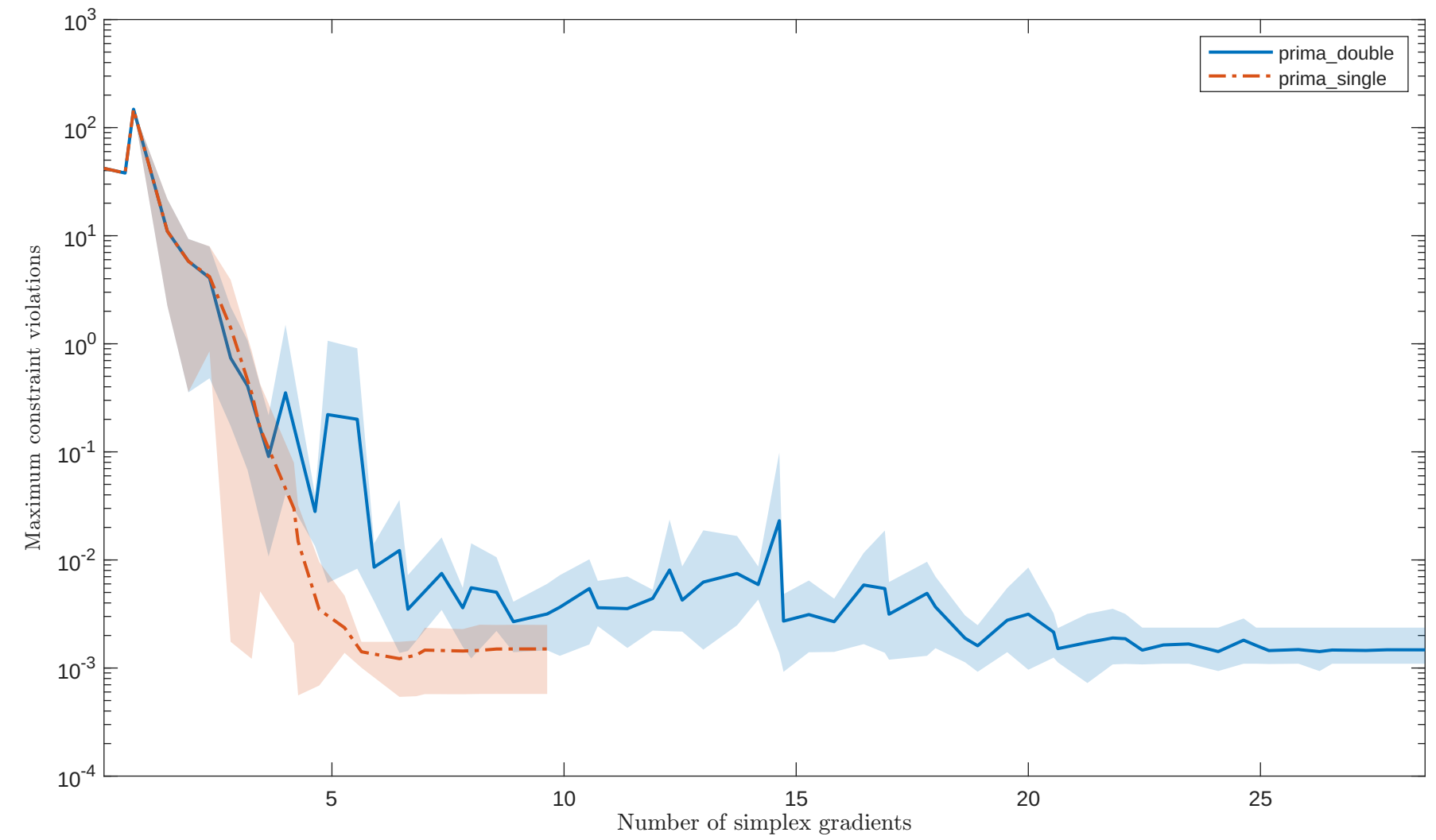
Solving "LUKVLE4" with "noisy_0.001_mixed_gaussian" feature
