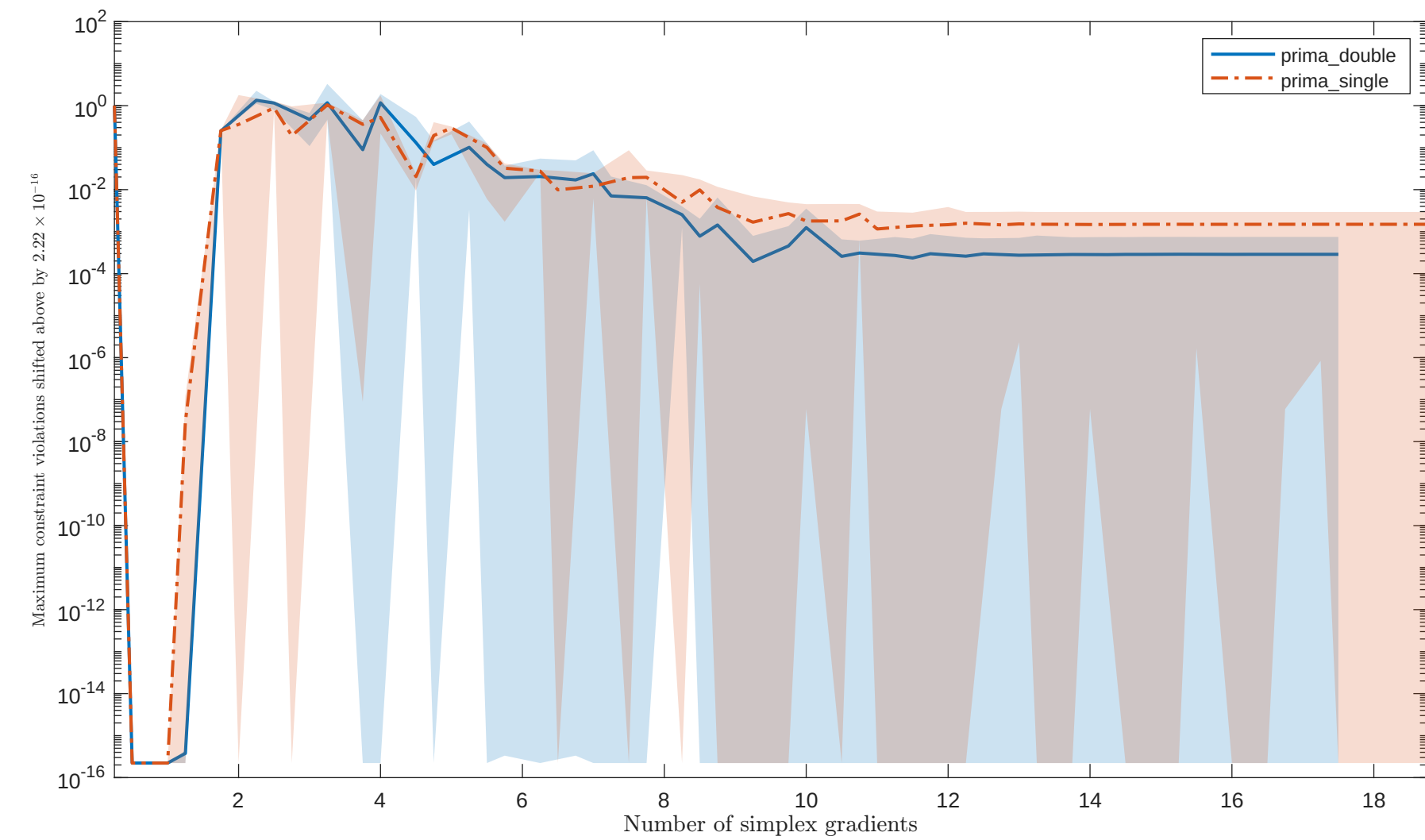
Solving "MAKELA1" with "noisy_0.001_mixed_gaussian" feature
