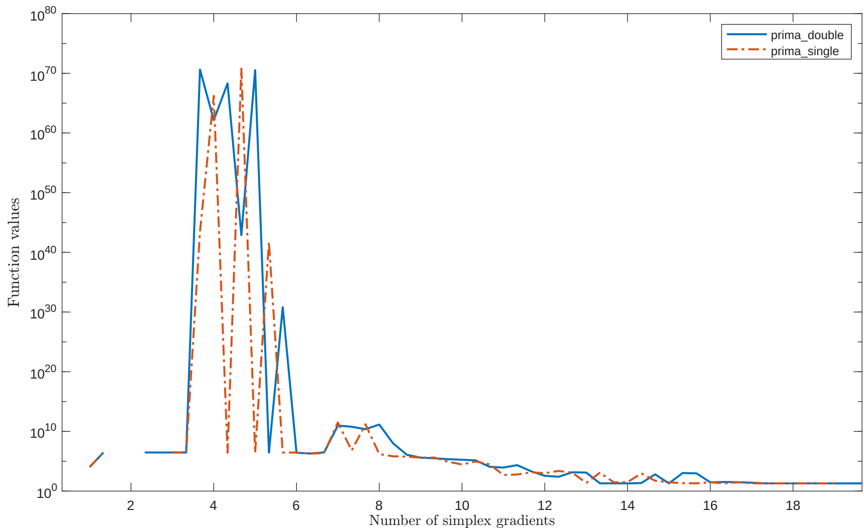
Solving "MISRA1ALS" with "noisy_0.001_mixed_gaussian" feature
