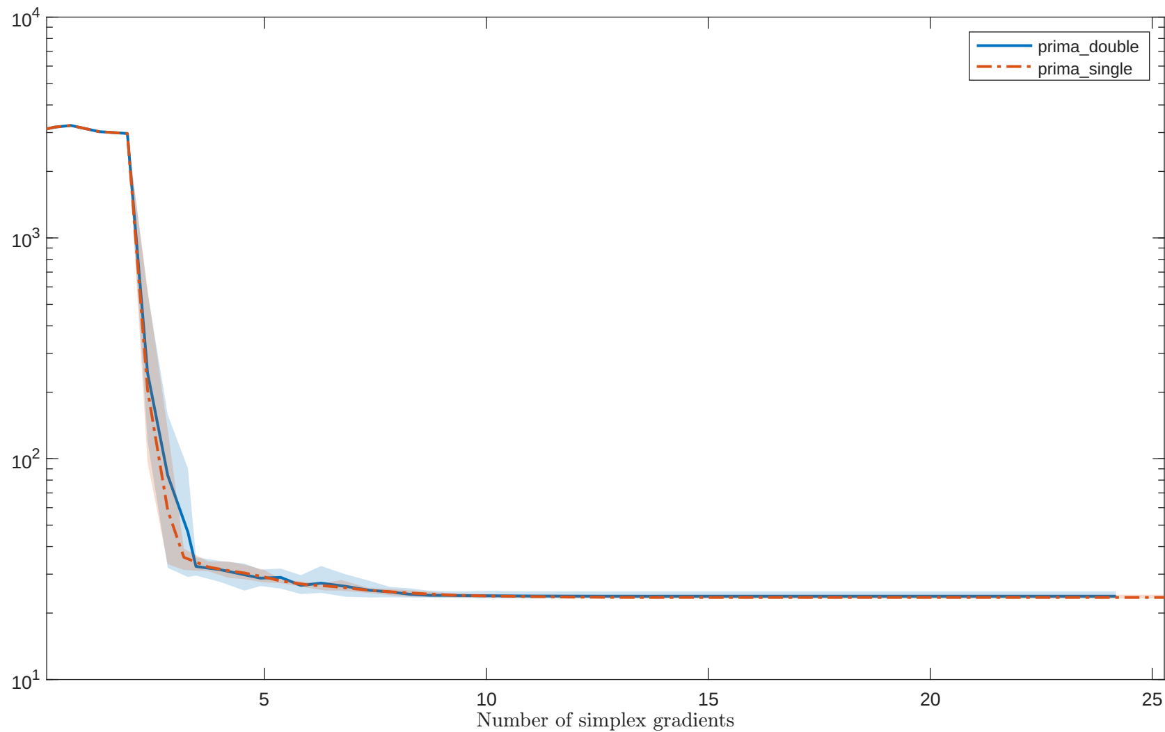
Solving "NONCVXU2" with "noisy_0.001_mixed_gaussian" feature
