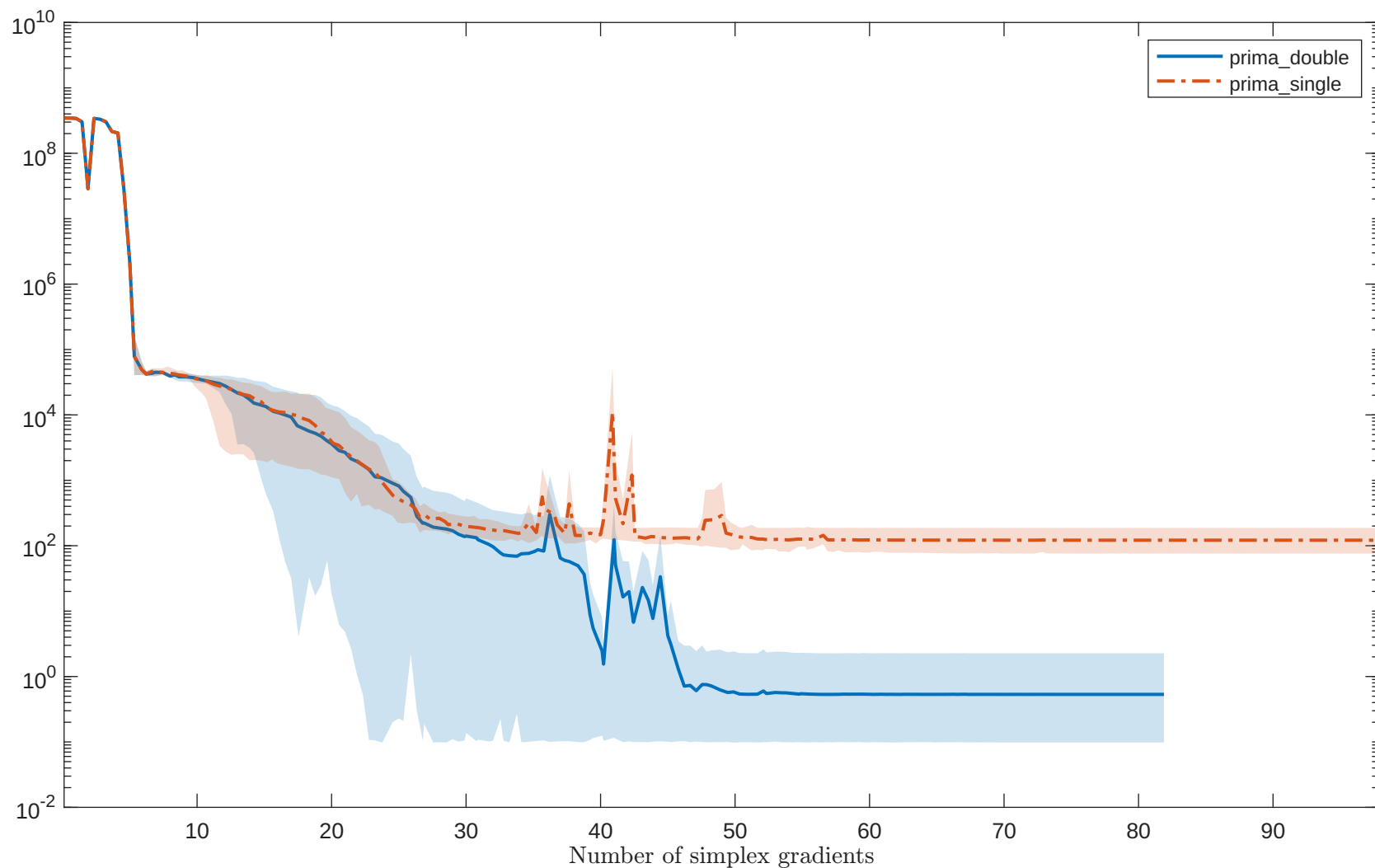
Solving "PALMER1C" with "noisy_0.001_mixed_gaussian" feature
