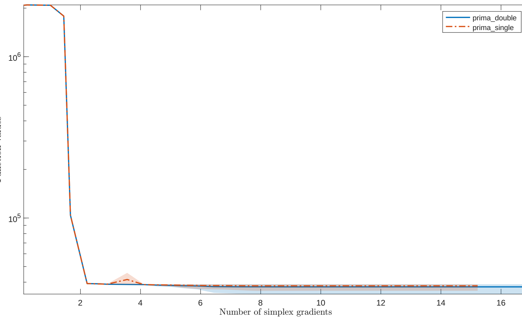
History profiles
