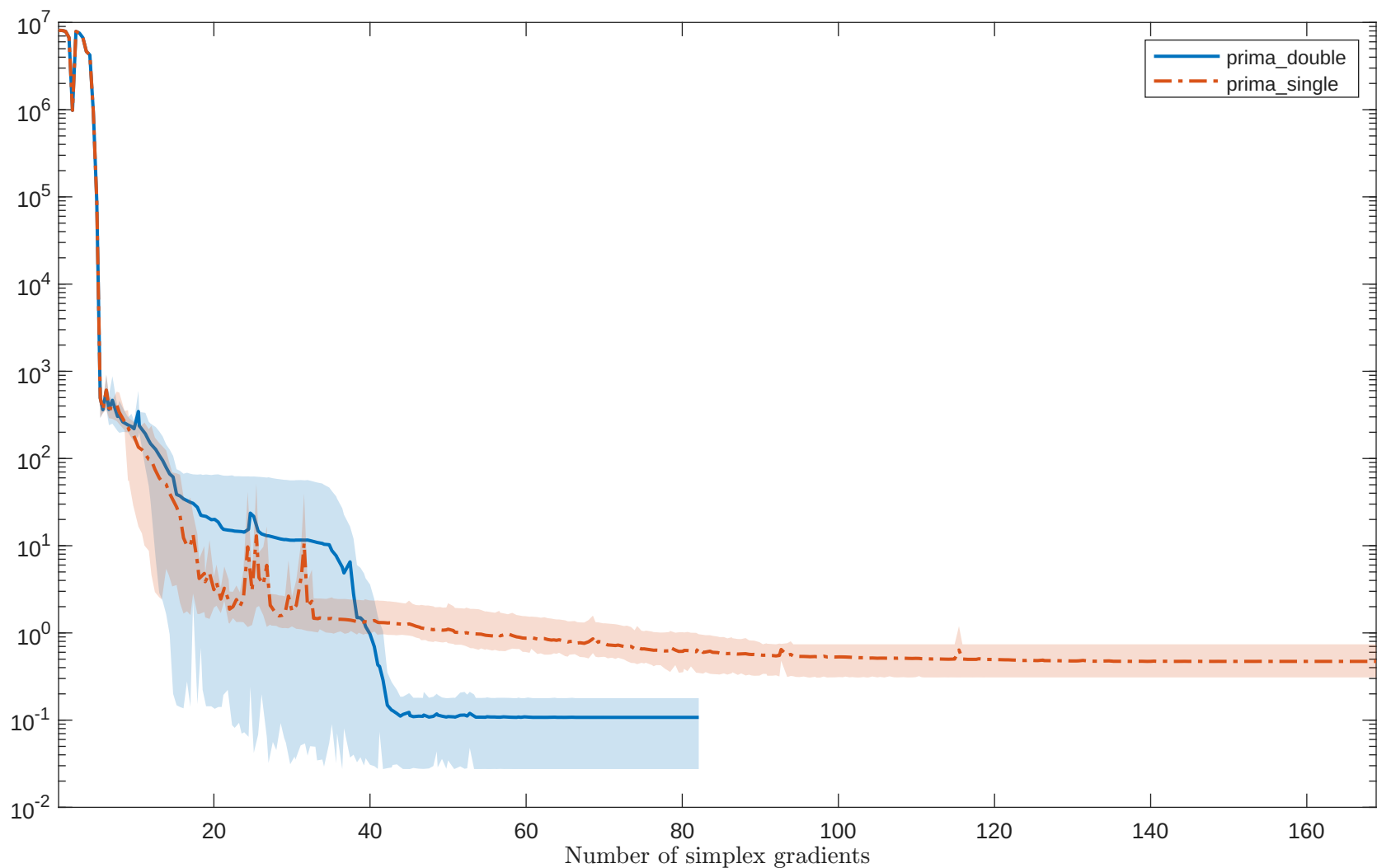
Solving "PALMER3C" with "noisy_0.001_mixed_gaussian" feature
