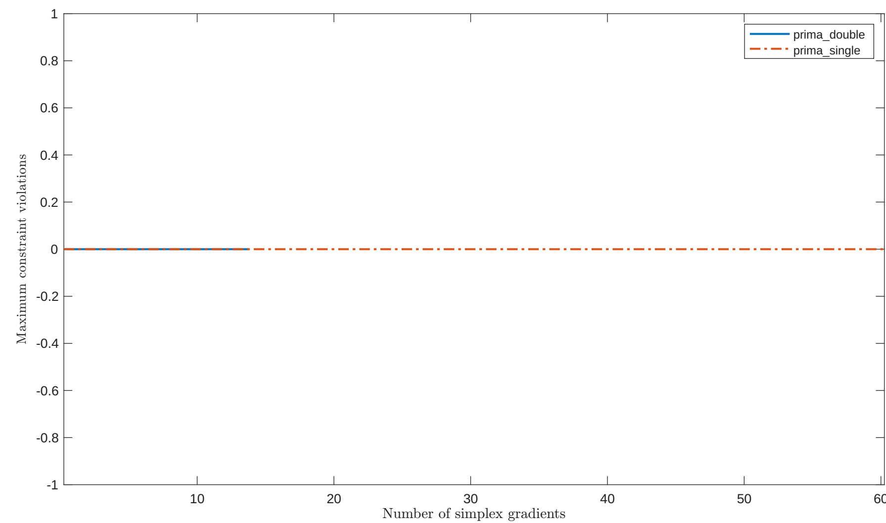
Solving "PFIT1LS" with "noisy_0.001_mixed.gaussian" feature
