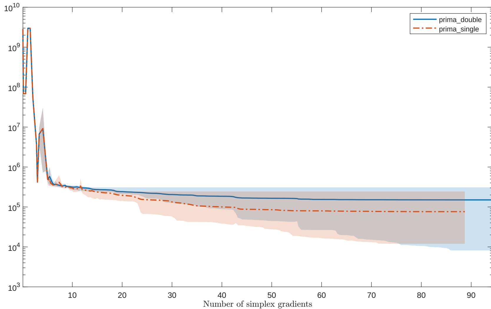
Solving "POWERSUM" with "noisy_0.001_mixed_gaussian" feature
