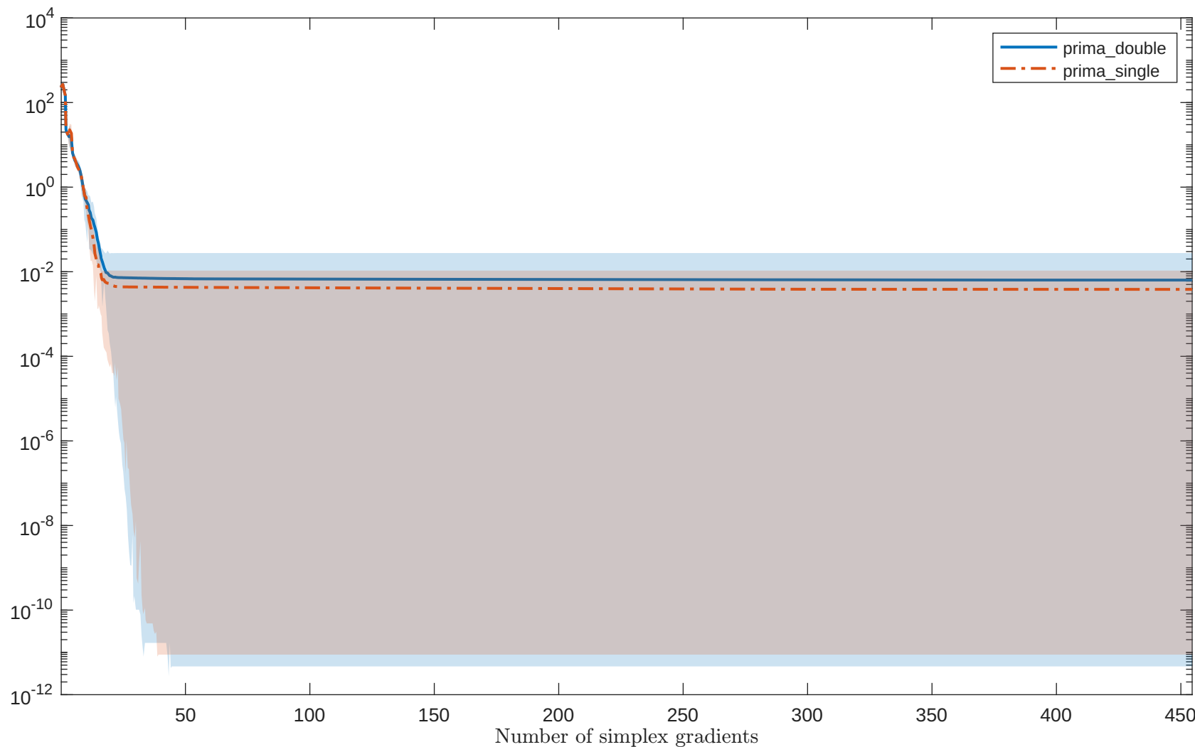
Solving “SPARSINE” with “noisy_0.001_mixed_gaussian” feature
