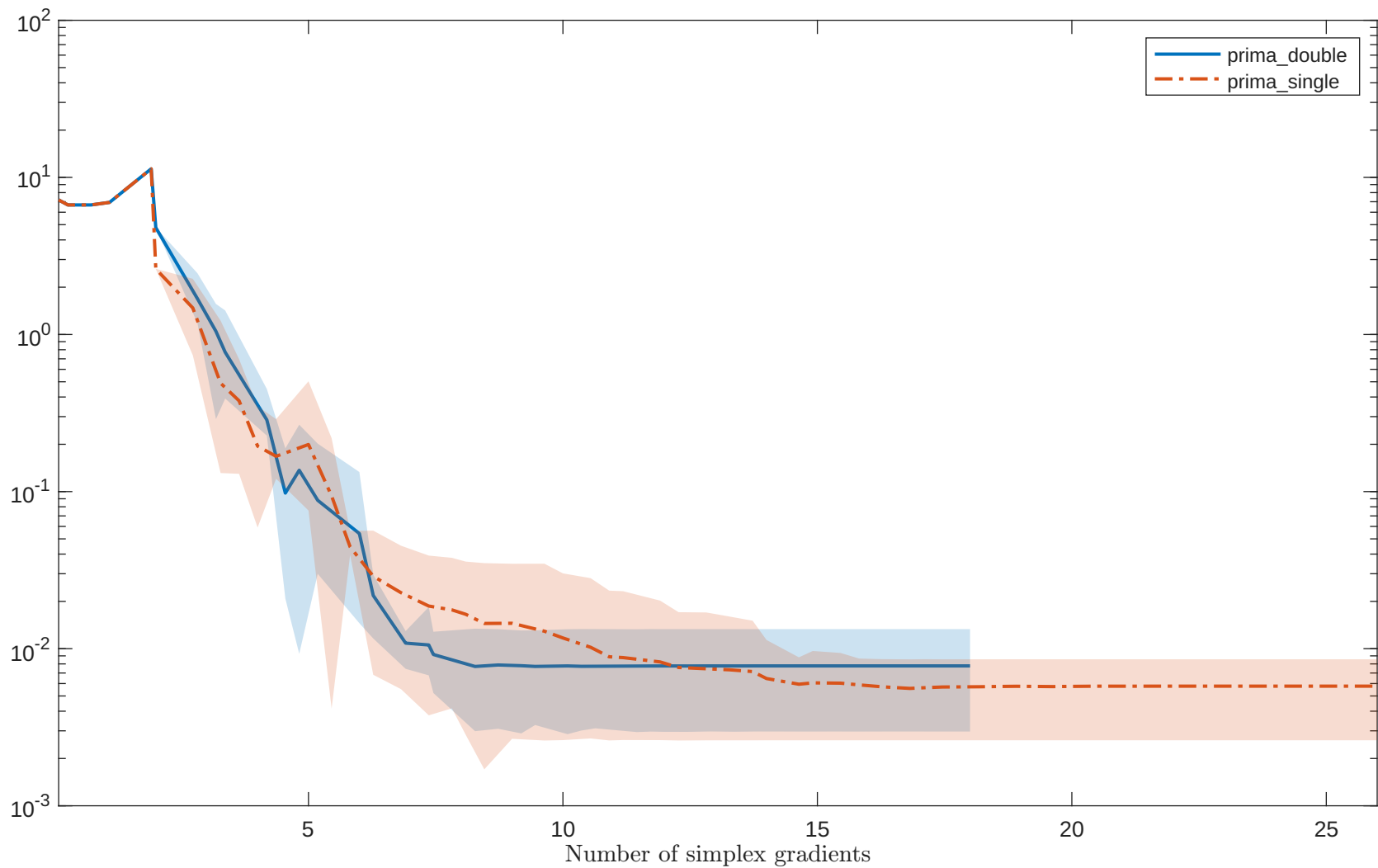
Solving "STRTCHDV" with "noisy_0.001_mixed_gaussian" feature
