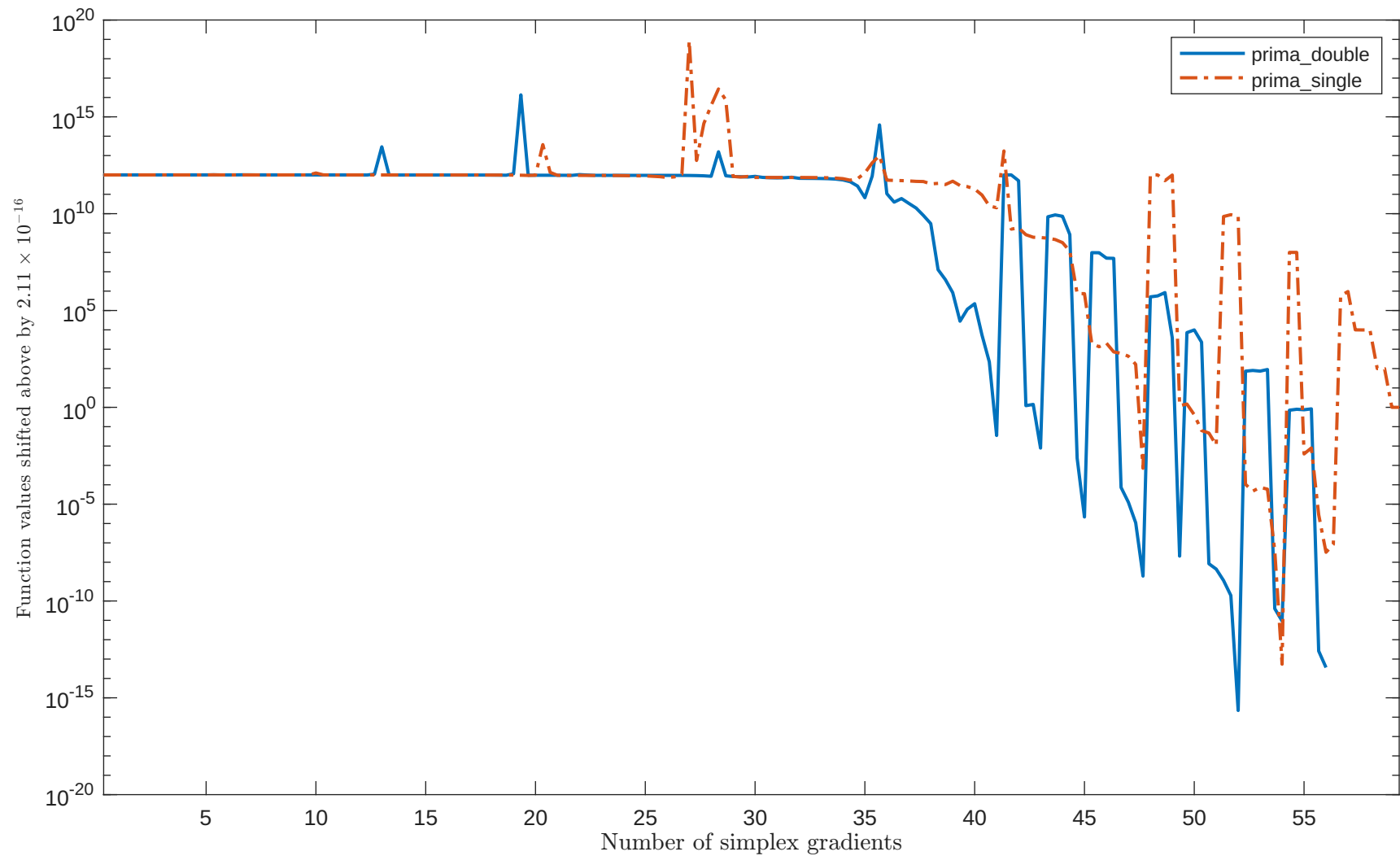
Solving "BROWNS" with "plain" feature
