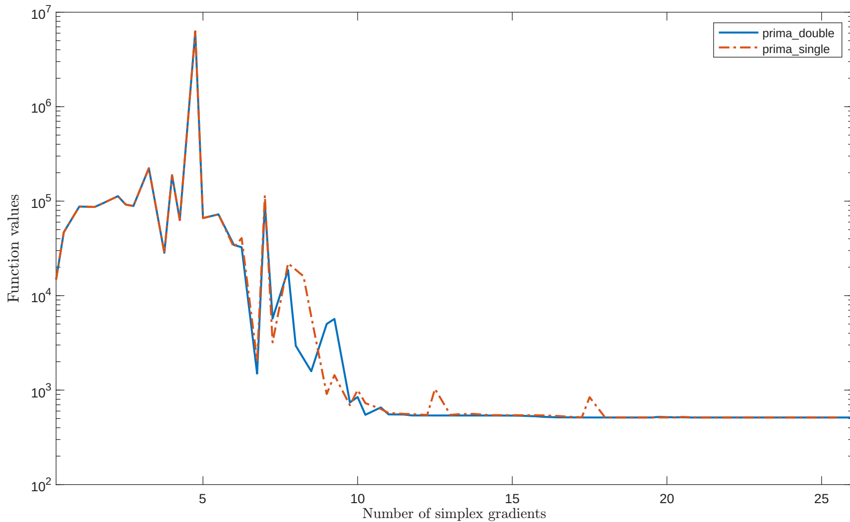
Solving "CHWIRUT2LS" with "plain" feature
