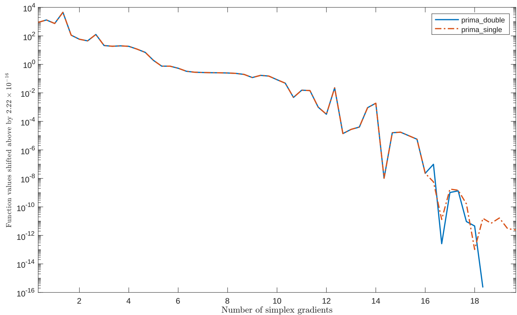
Solving "DENSCHNC" with "plain" feature
