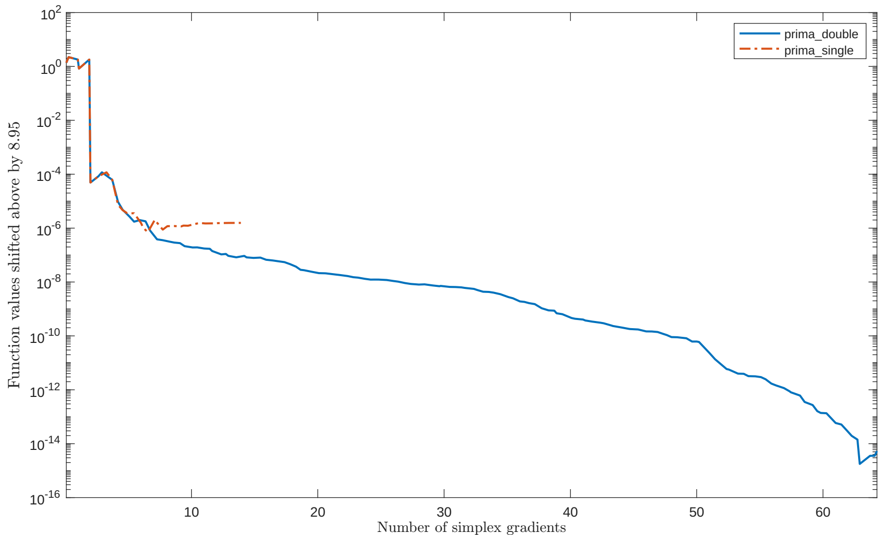
Solving “EG2” with “plain” feature
