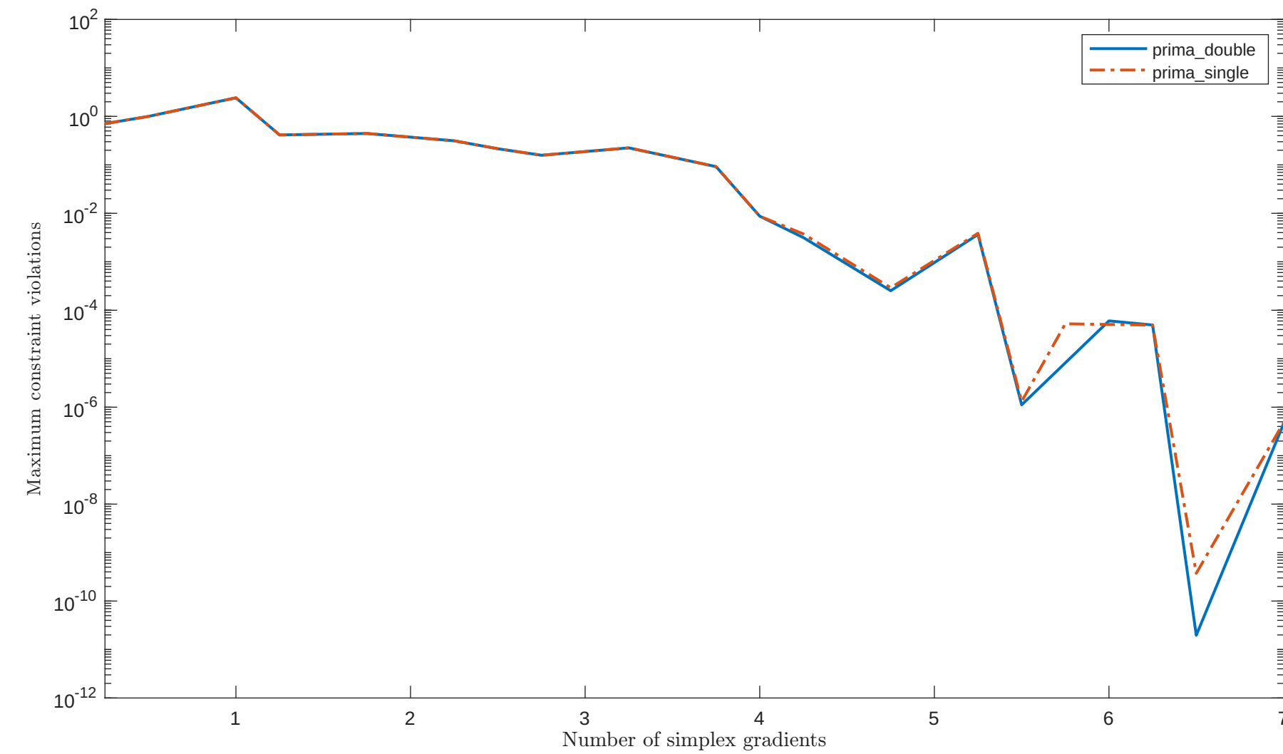
Solving "EIGMAXA" with "plain" feature
