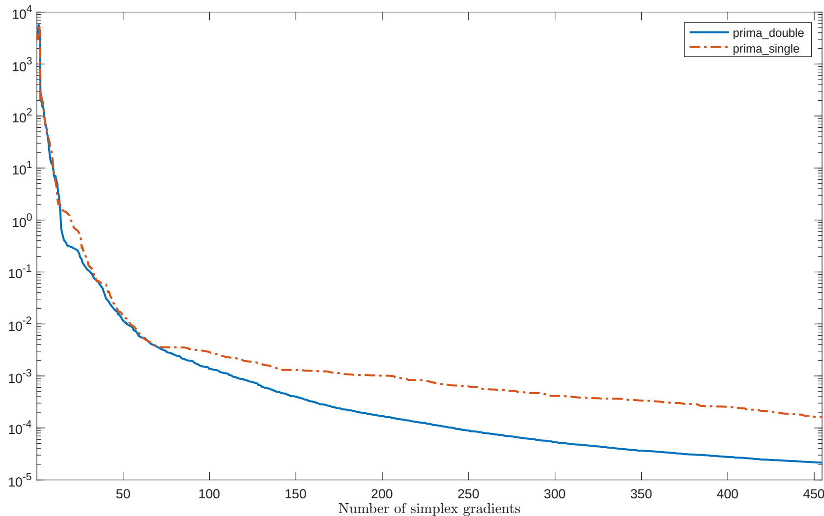
Solving "EXTROSNB" with "plain" feature
