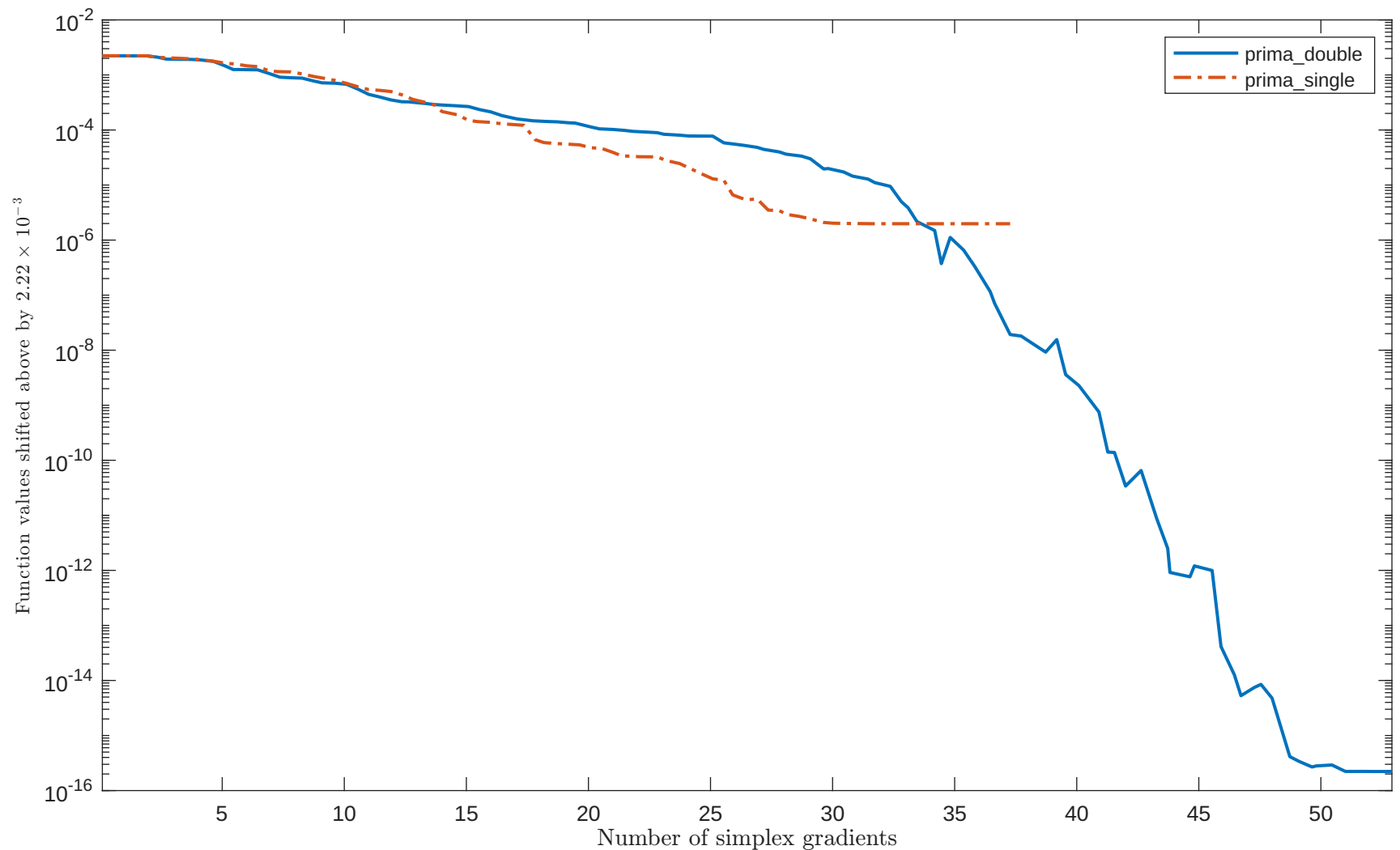
Solving “FLETBV3M” with “plain” feature
