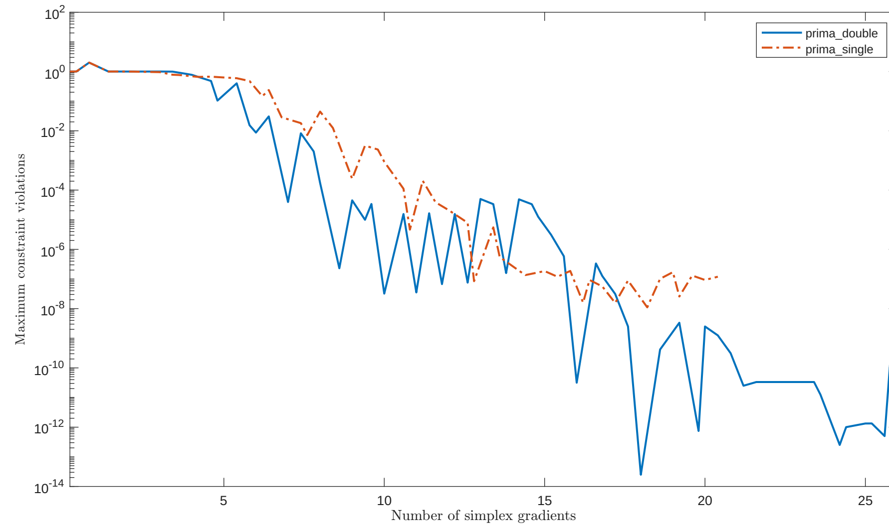
Solving "FLETCHER" with "plain" feature
