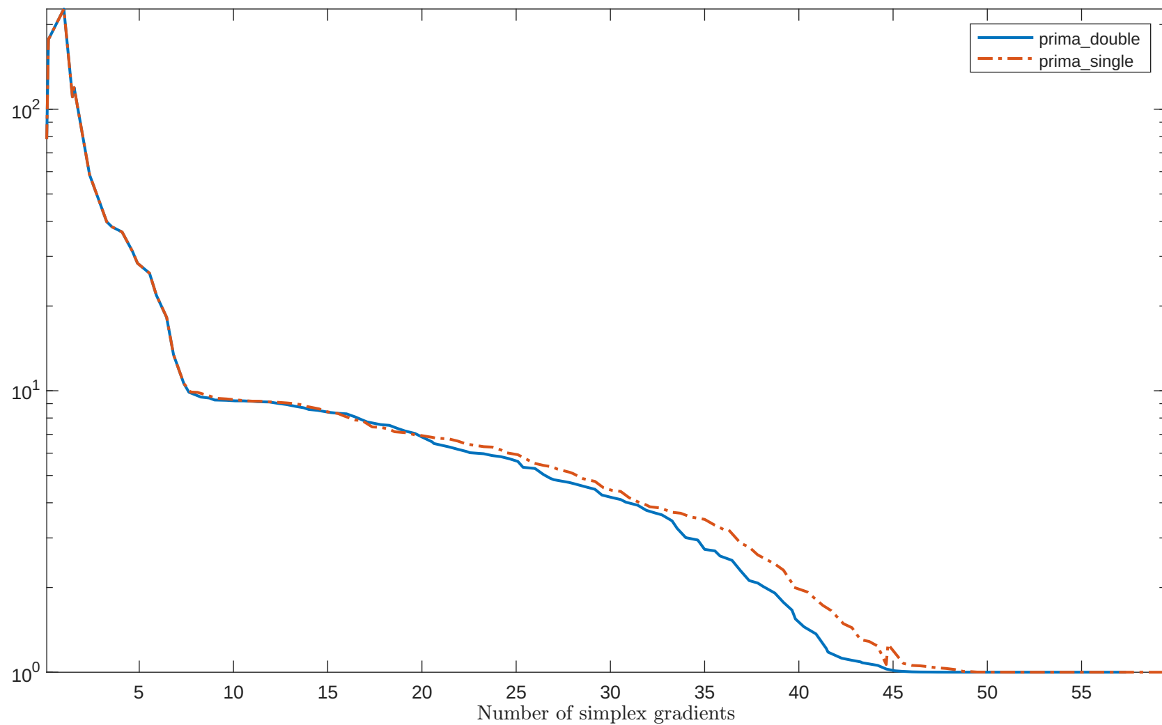
Solving "GENROSE" with "plain" feature
