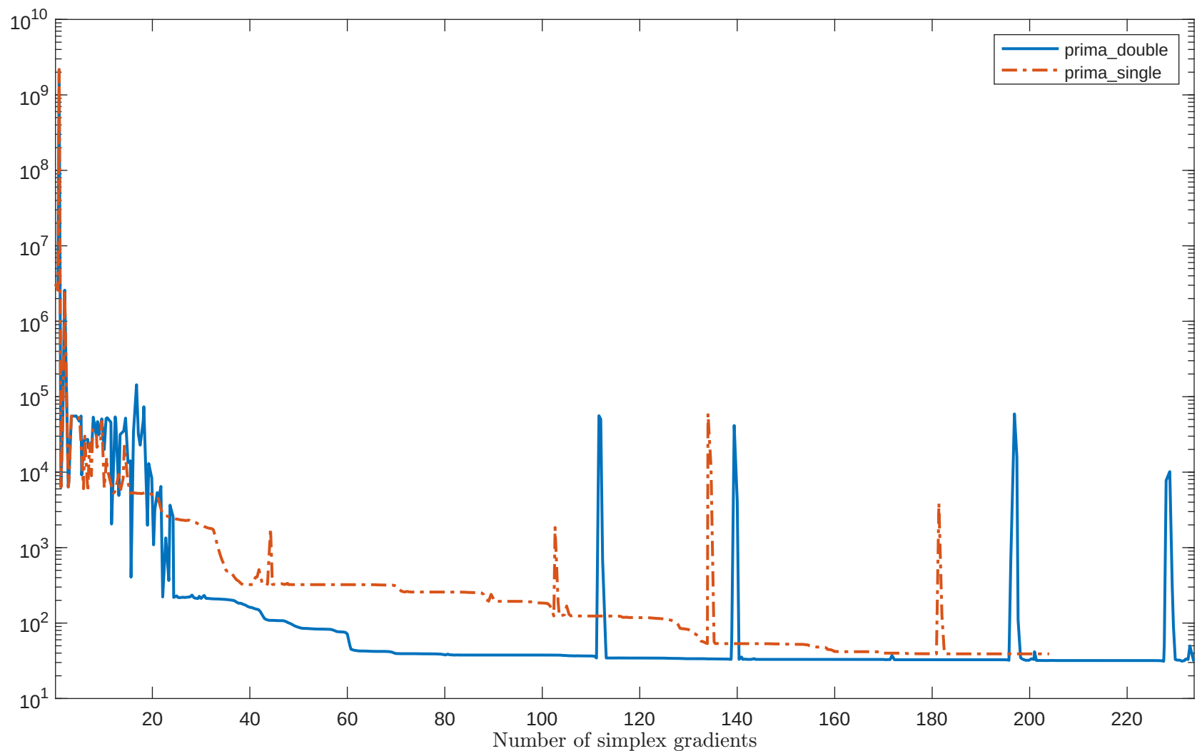
Solving "HAHN1LS" with "plain" feature
