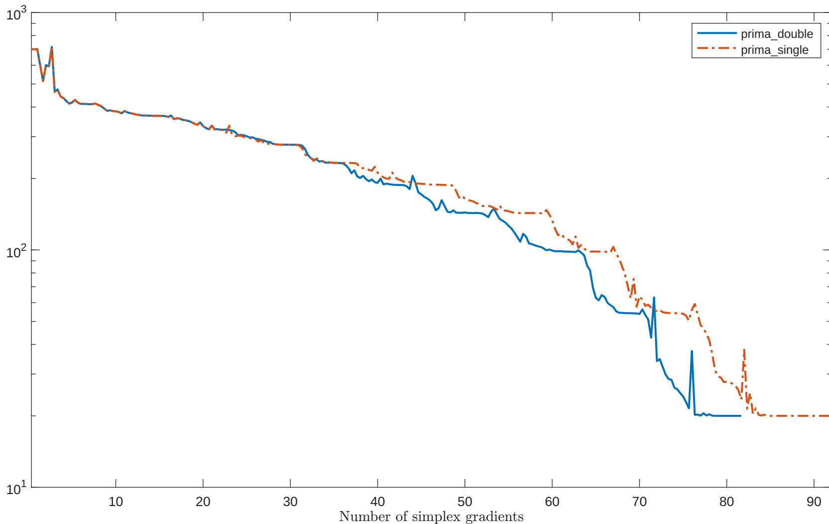
Solving "HAIRY" with "plain" feature
