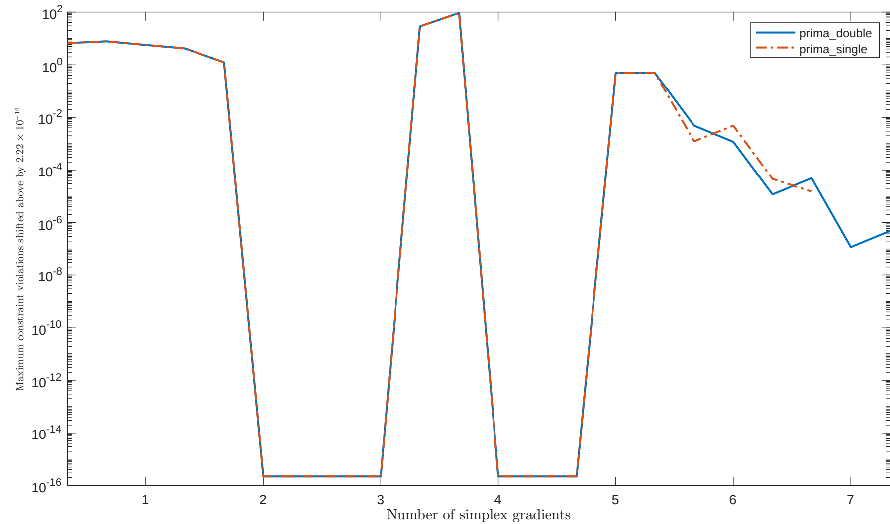
Solving "HIMMELP5" with "plain" feature
