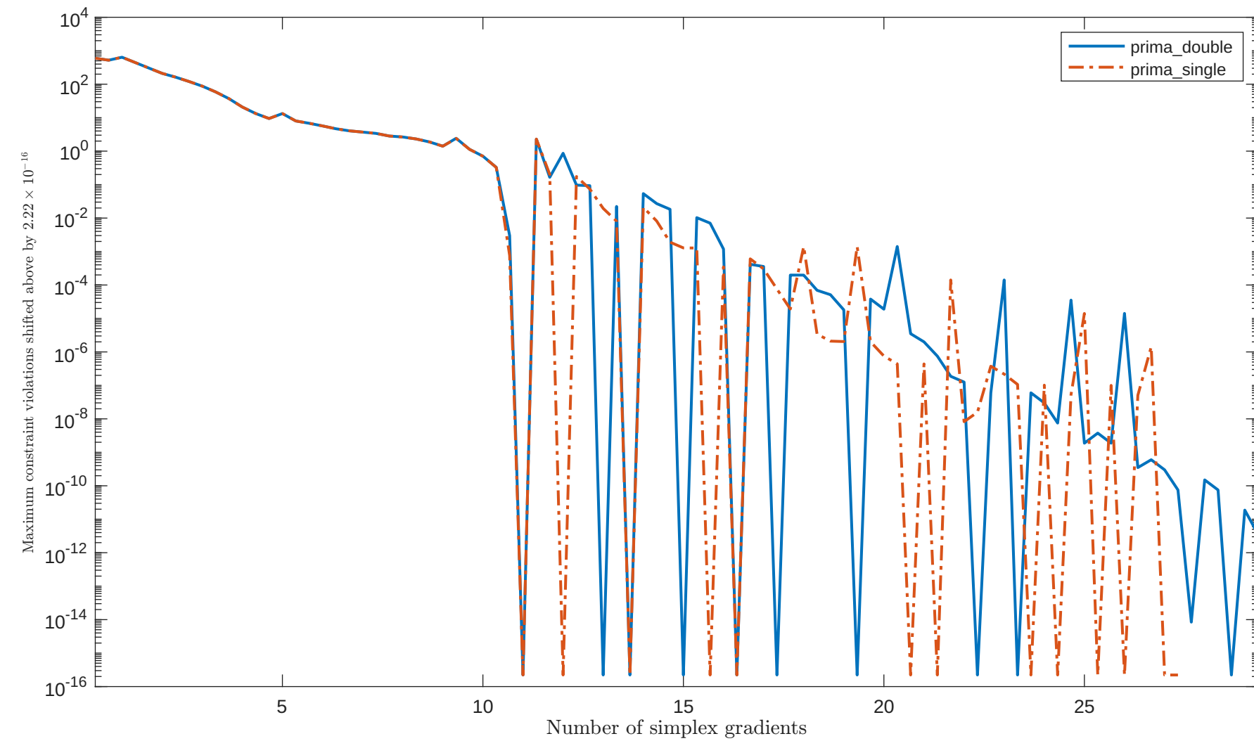
Solving "HS10" with "plain" feature
