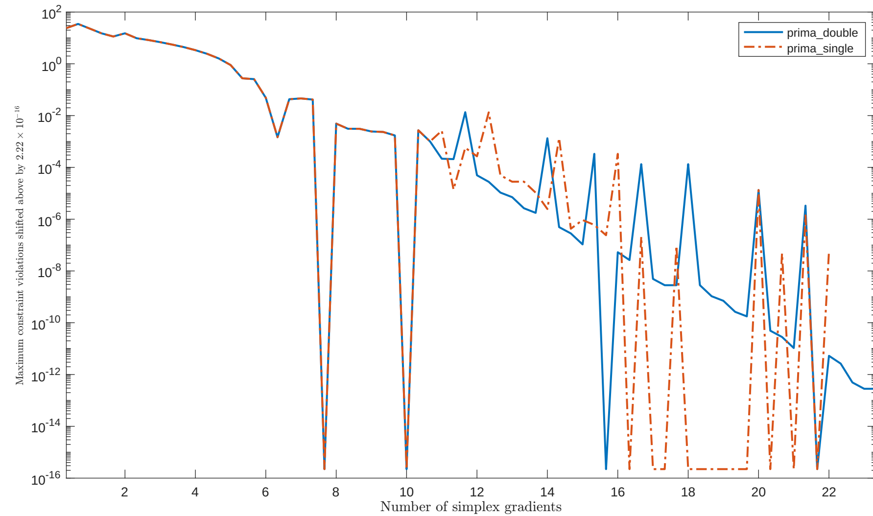
Solving "HS11" with "plain" feature
