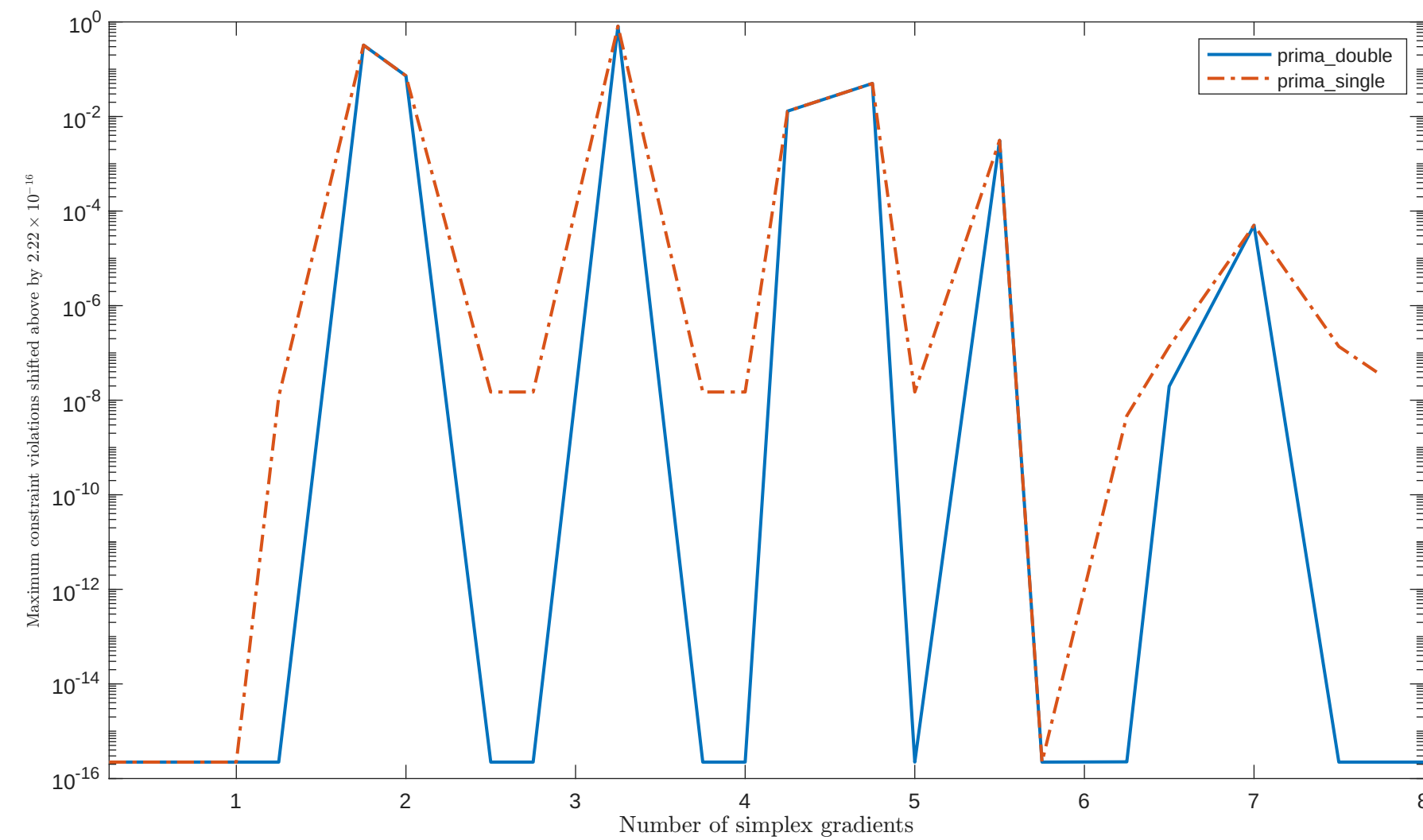
Solving "HS33" with "plain" feature
