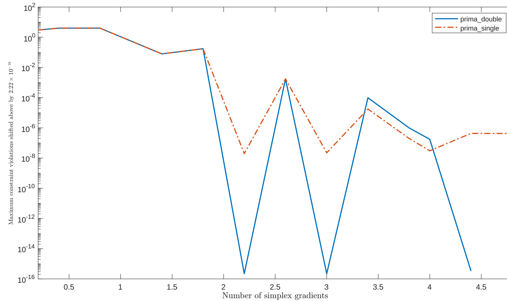
Solving "HS73" with "plain" feature
