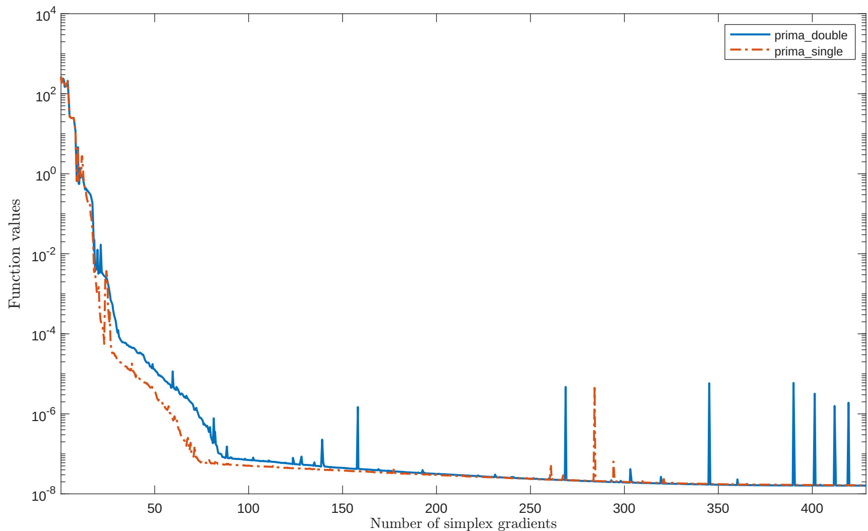
Solving “LANCZOS3LS” with “plain” feature
