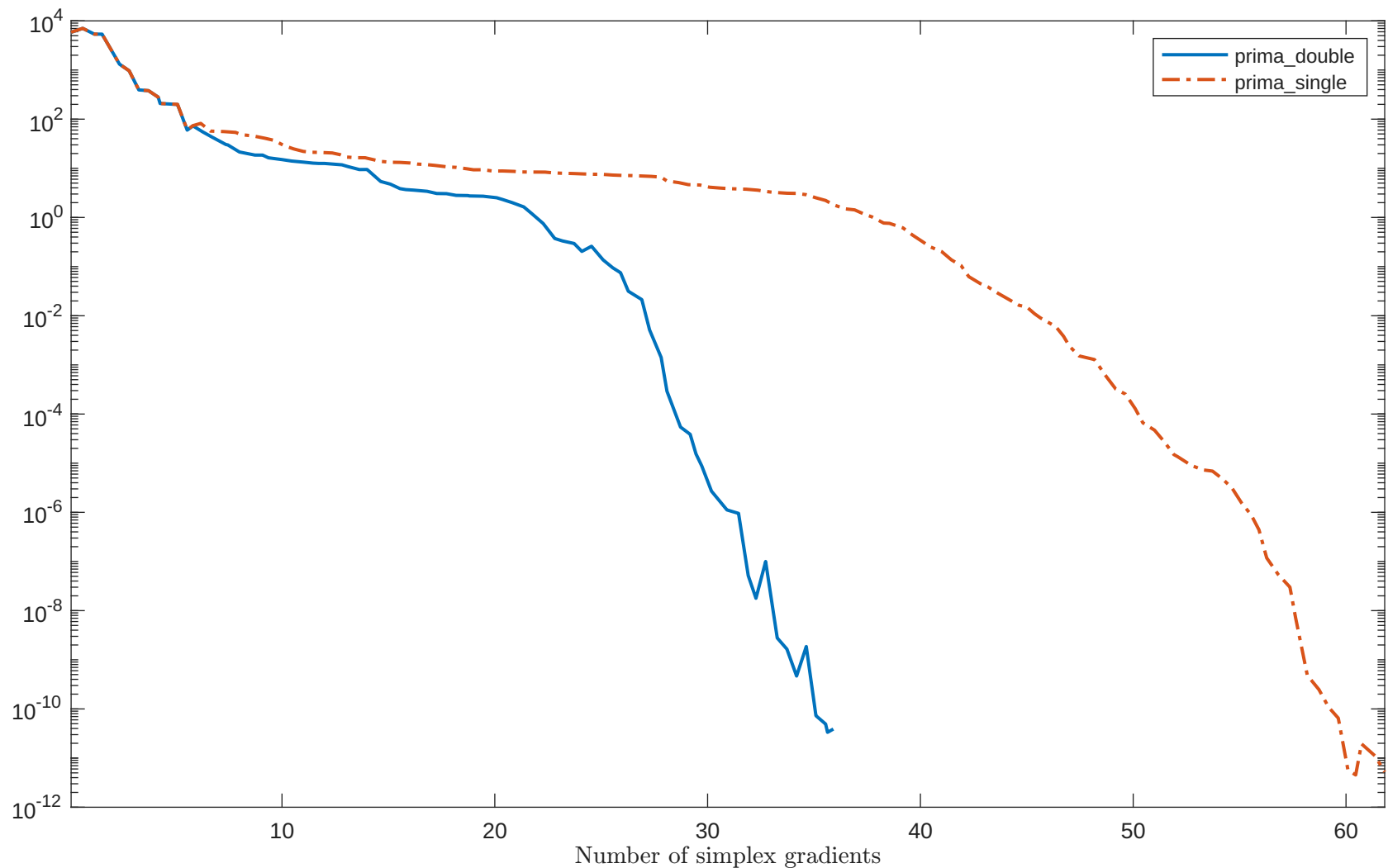
Solving "LIARWHD" with "plain" feature
