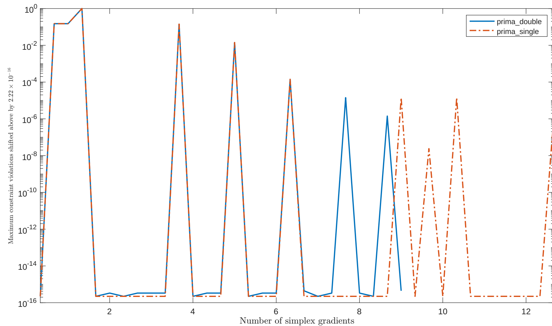
Solving "LSQFIT" with "plain" feature
