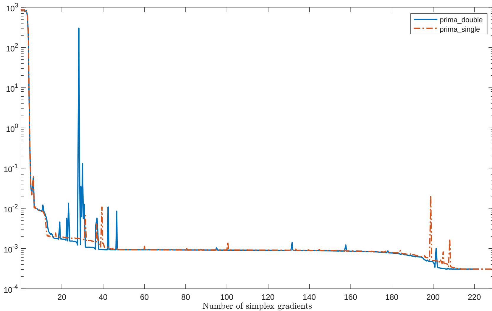
Solving “MGH09LS” with “plain” feature
