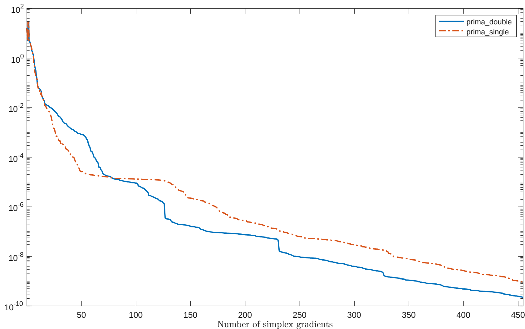
Solving "NONDQUAR" with "plain" feature
