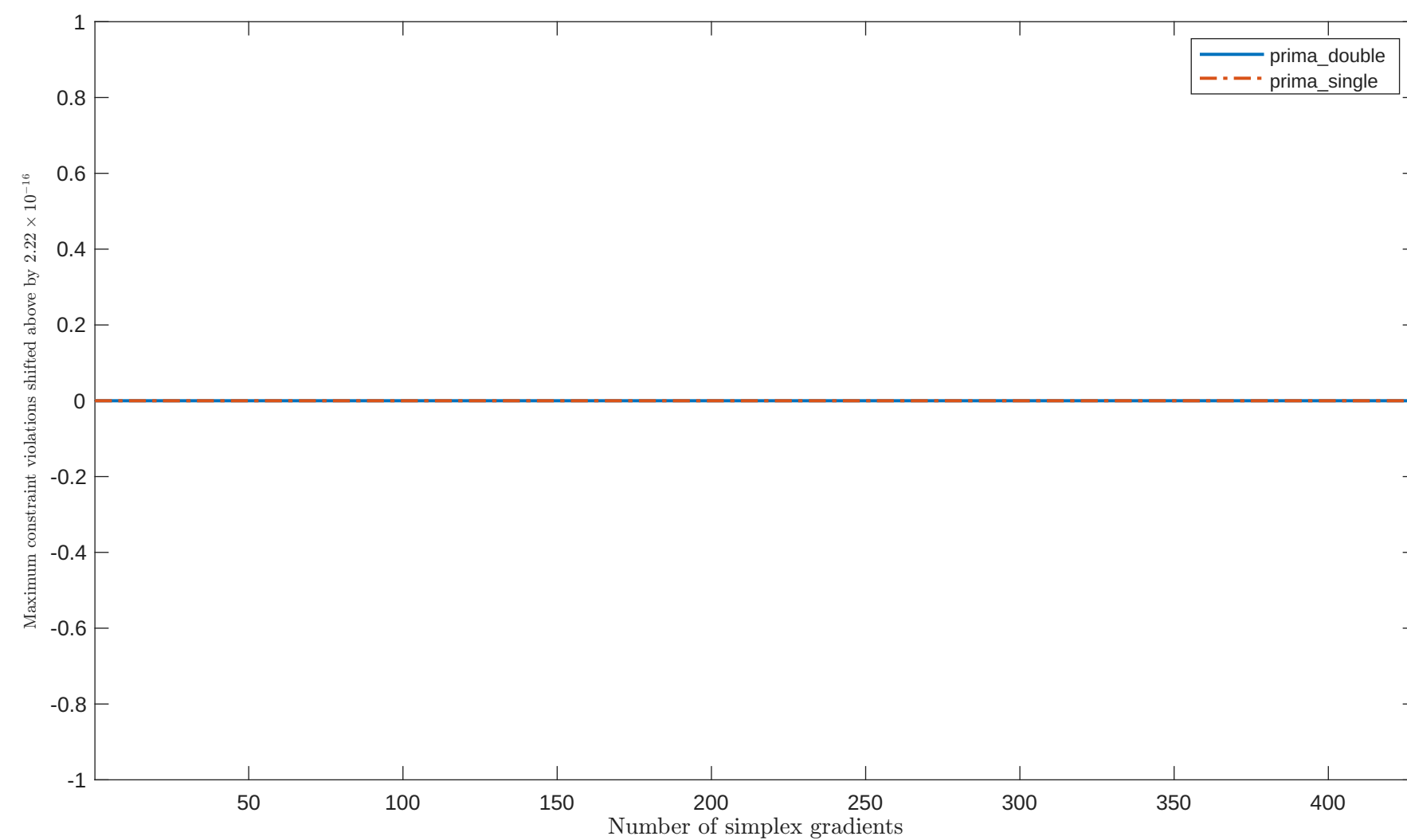
Solving "PALMER2A" with "plain" feature
