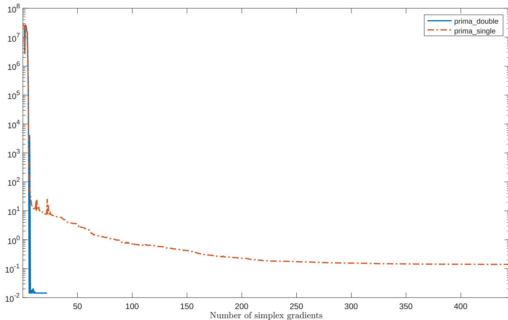
Solving "PALMER2C" with "plain" feature
