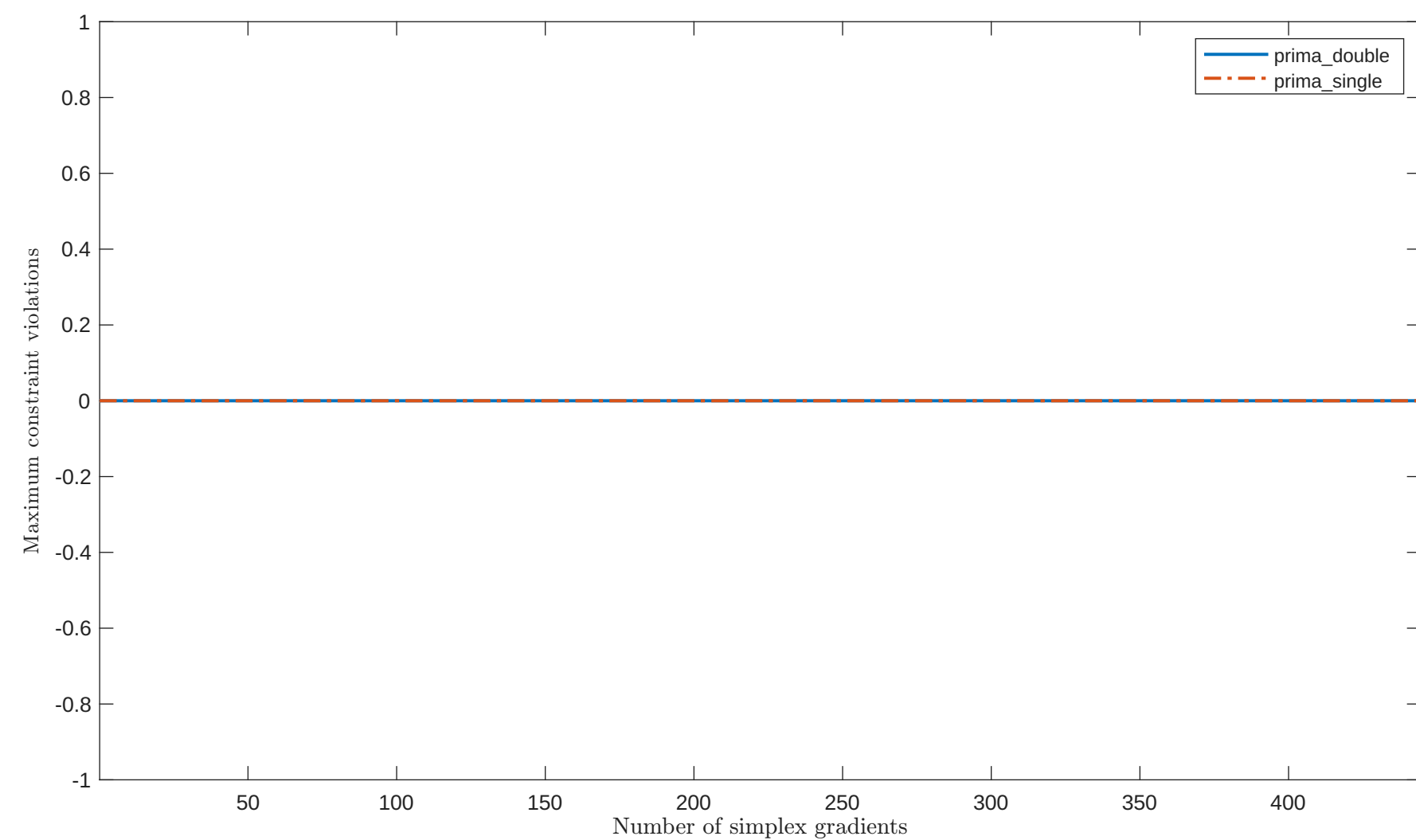
Solving "PALMER6E" with "plain" feature
