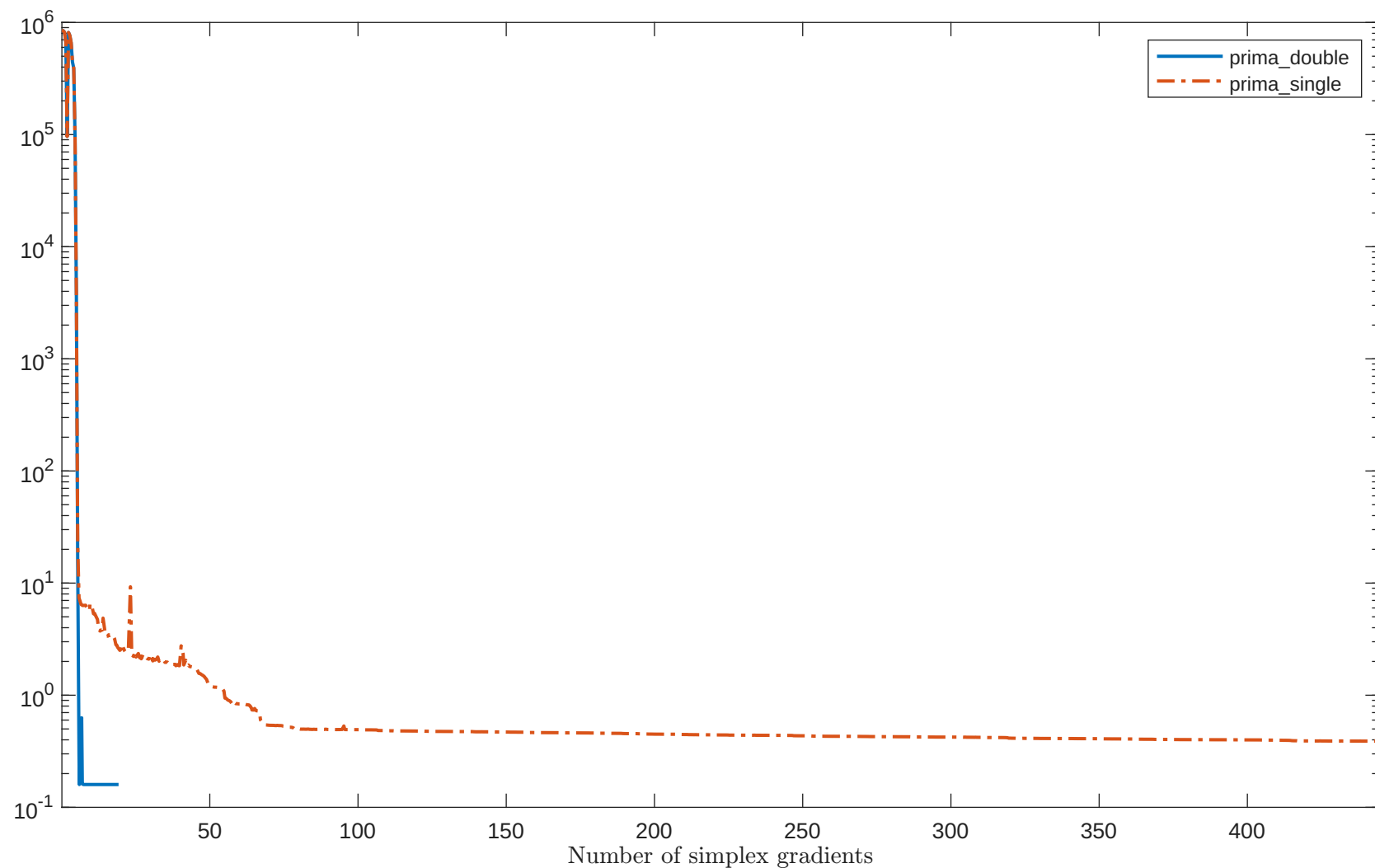
Solving "PALMER8C" with "plain" feature
