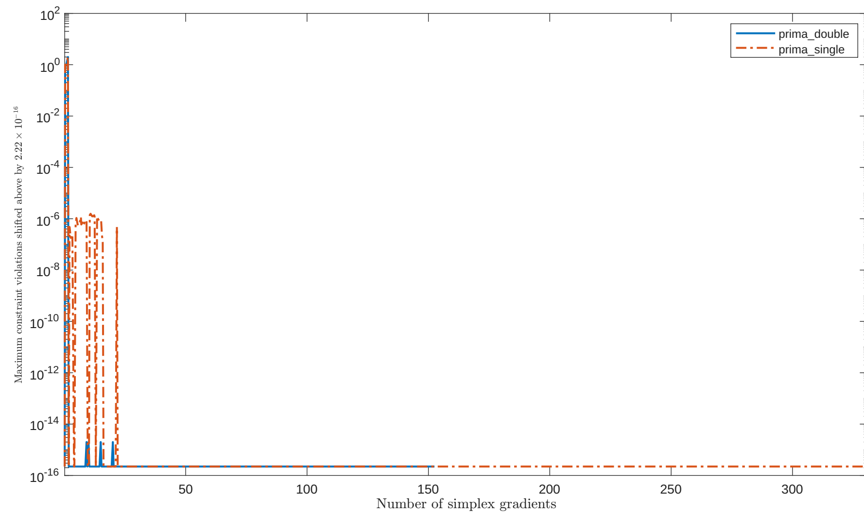
Solving "S268" with "plain" feature
