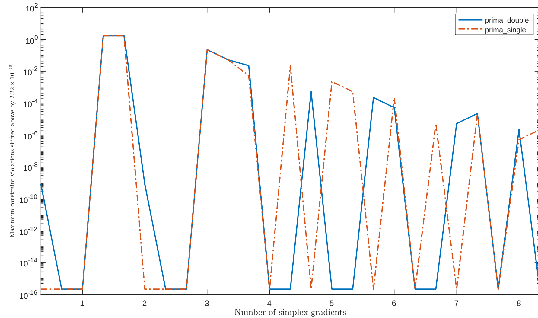
Solving "SIMPLLPB" with "plain" feature
