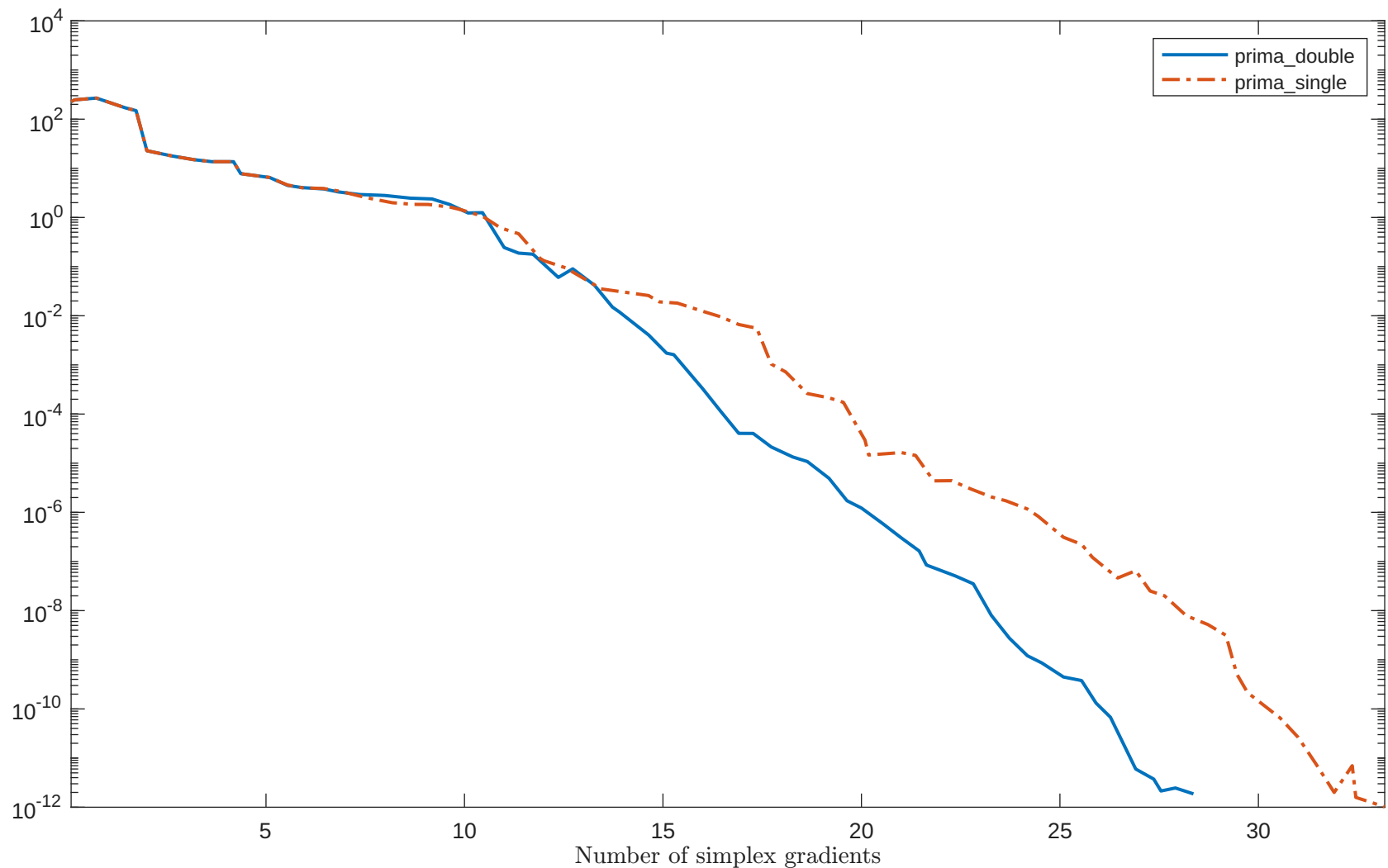
Solving "SPARSINE" with "plain" feature
