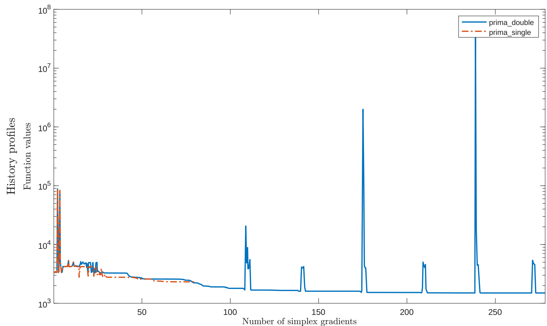
Solving “VESUVIALS” with “plain” feature
