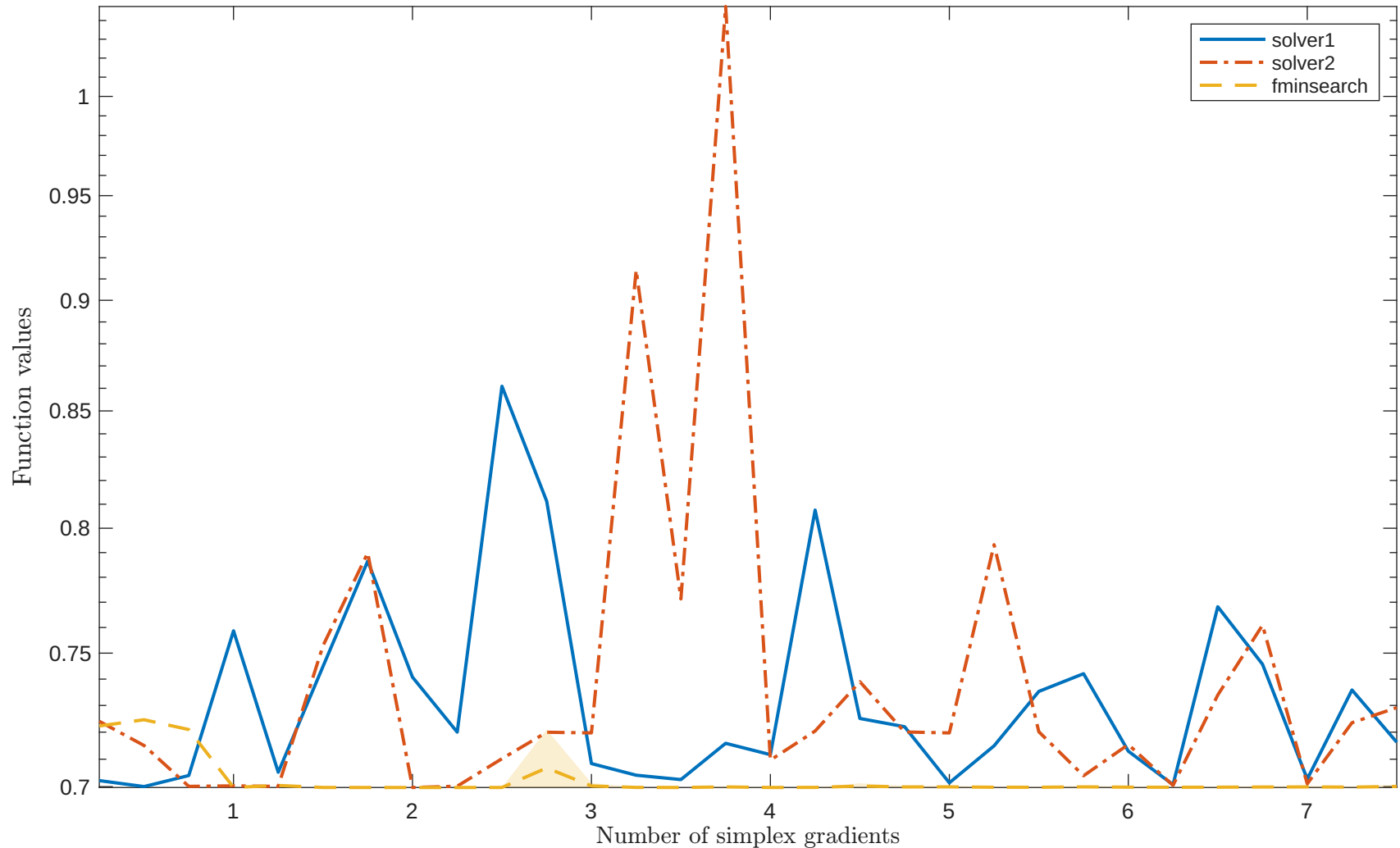
Solving "ECKERLE4LS" with "noisy_0.001_mixed_gaussian" feature
